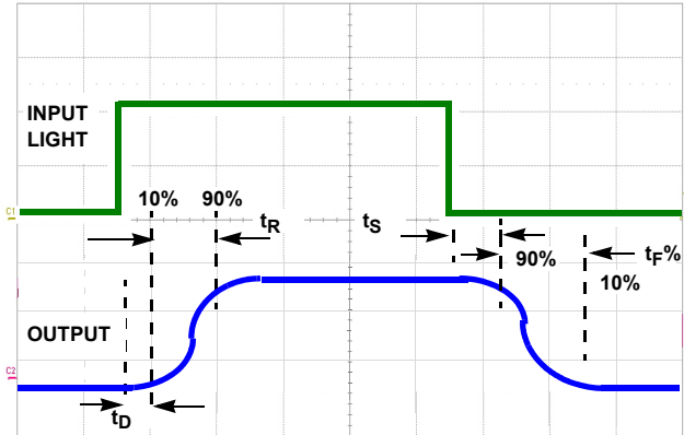
FIGURE 2. TIMING DIAGRAM
