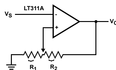
FIGURE 10. COMPARATOR WITH HYSTERESIS
