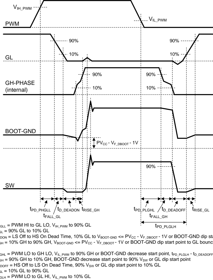
Figure 24. PWM Timing Diagram
