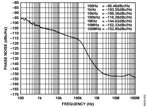
Figure 52. LO Phase Noise vs. Frequency Offset, LO = 525 MHz, PLL Loop Bandwidth = 50 kHz
