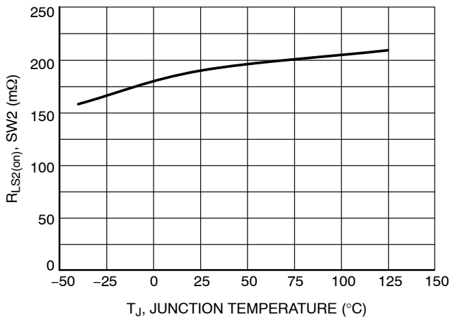
Figure 15. SW2 Low Side R DS(on) vs. Junction Temperature
