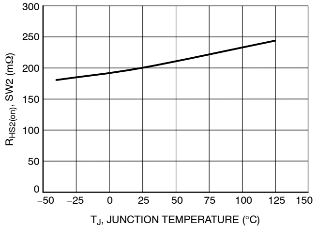
Figure 14. SW2 High Side R DS(on) vs. Junction Temperature
