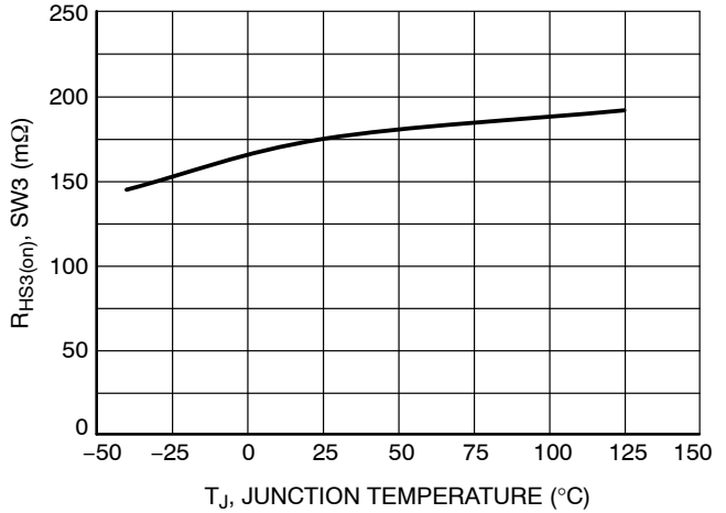
Figure 16. SW3 High Side R DS(on) vs. Junction Temperature
