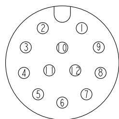
Pin Assignments
