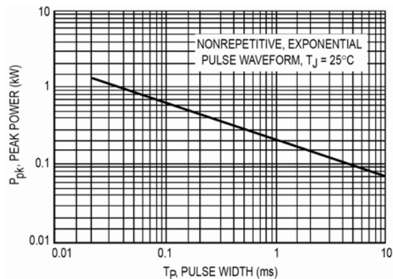
Figure 8. Typical pulse rating curve
