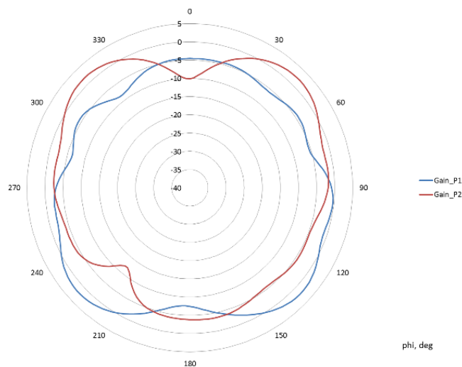
Horizontal plane
