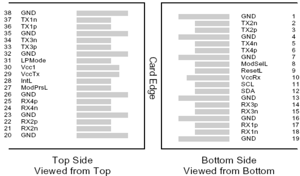
Figure 1 – QSFPP MSA-compliant 38-pin connector
