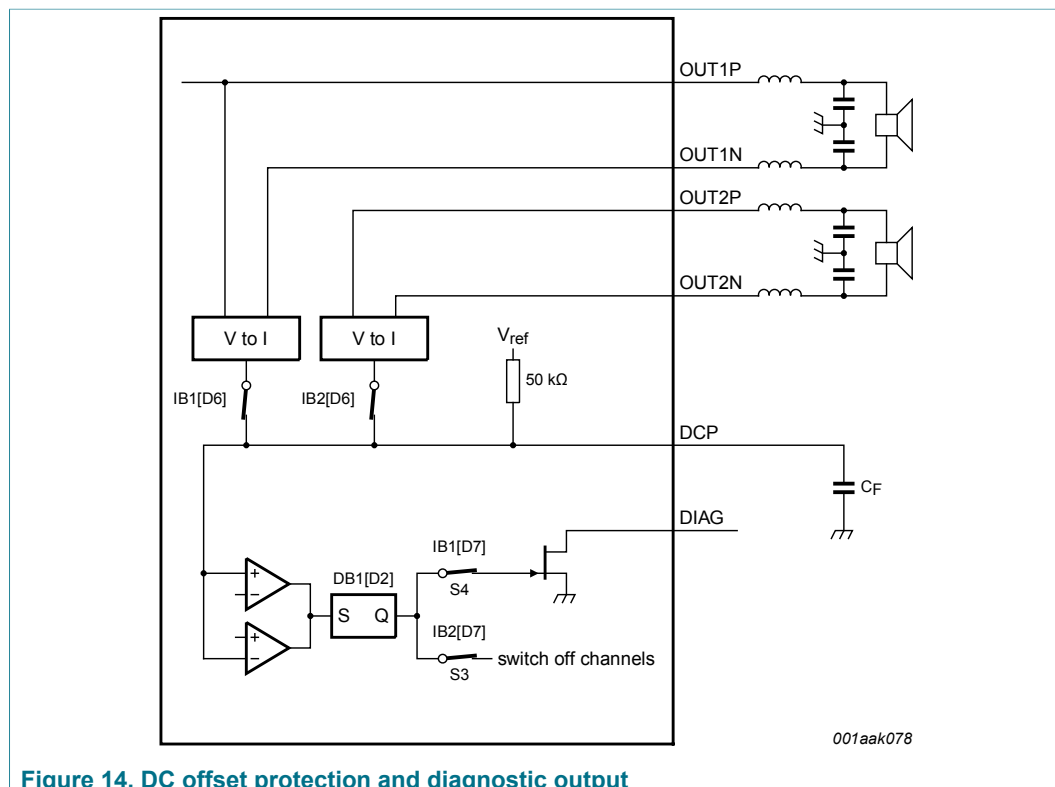
Figure 14. DC offset protection and diagnostic output
