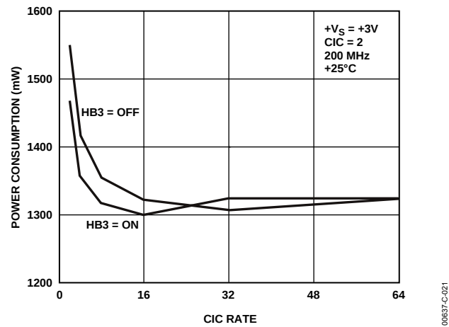
Figure 21. Power Consumption vs. CIC Rate; V_S = 3\text{ V} , 200\text{ MHz} , 2^\circ\text{C}
