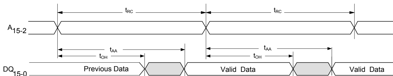
Figure 5. Read Cycle Timing 1 ( \overline{\text{CE}} LOW, \overline{\text{OE}} LOW)
