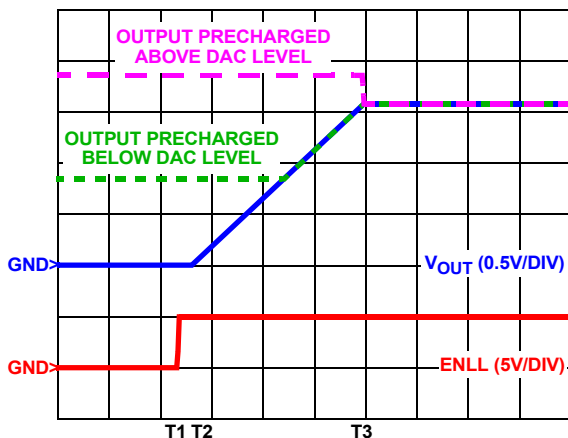
FIGURE 12. SOFT-START WAVEFORMS FOR ISL6308A-BASED MULTI-PHASE CONVERTER
