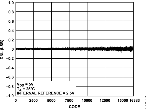
Figure 16. AD5695R DNL
