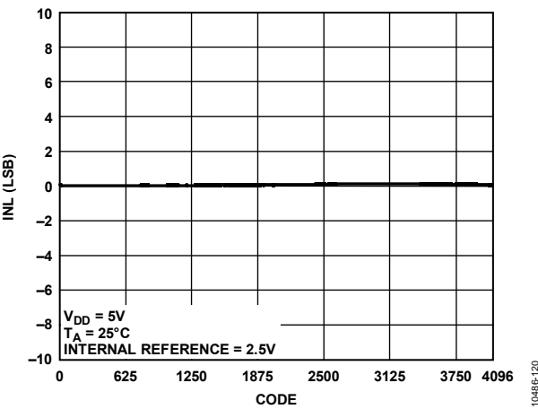
Figure 14. AD5694R INL
