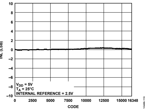
Figure 13. AD5695R INL
