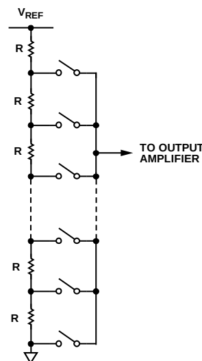
Figure 46. Resistor String Structure
