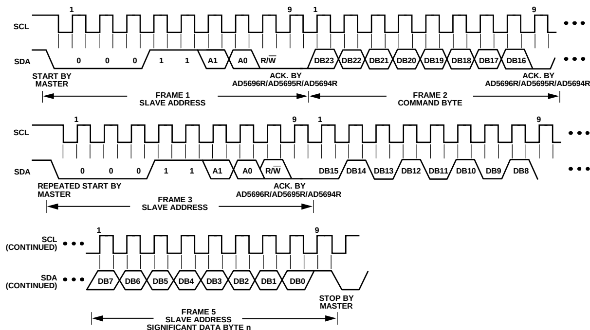
Figure 51. I²C Read Operation
