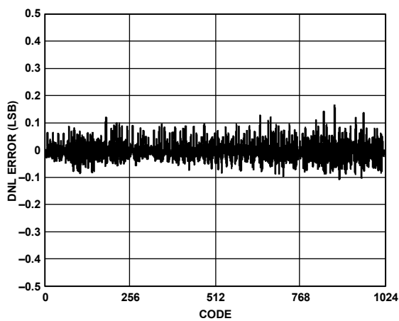
Figure 17. Typical DNL for the AD7441
