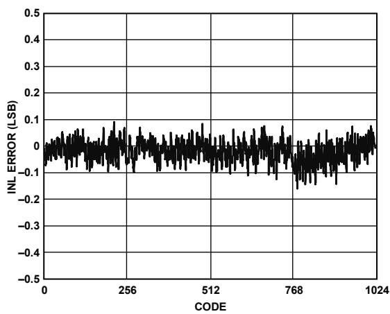
Figure 18. Typical INL for the AD7441
