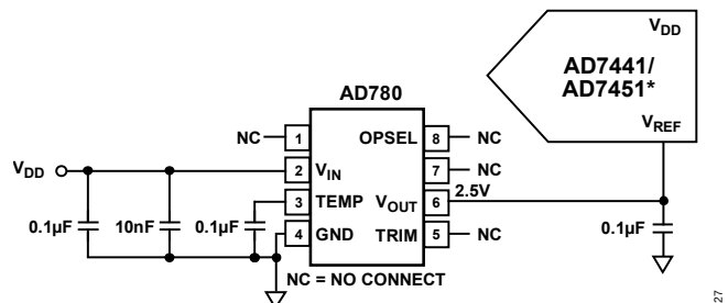
Figure 27. Typical V_{REF} Connection Diagram for V_{DD} = 5\text{ V}
