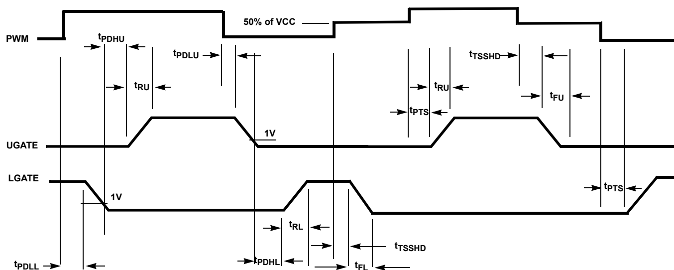
FIGURE 3. TIMING DIAGRAM
