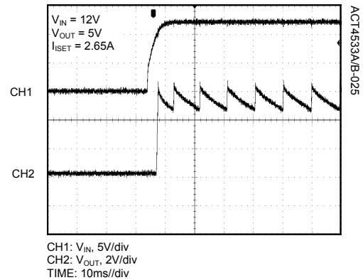
OVP Test (Start up with FB=0)
