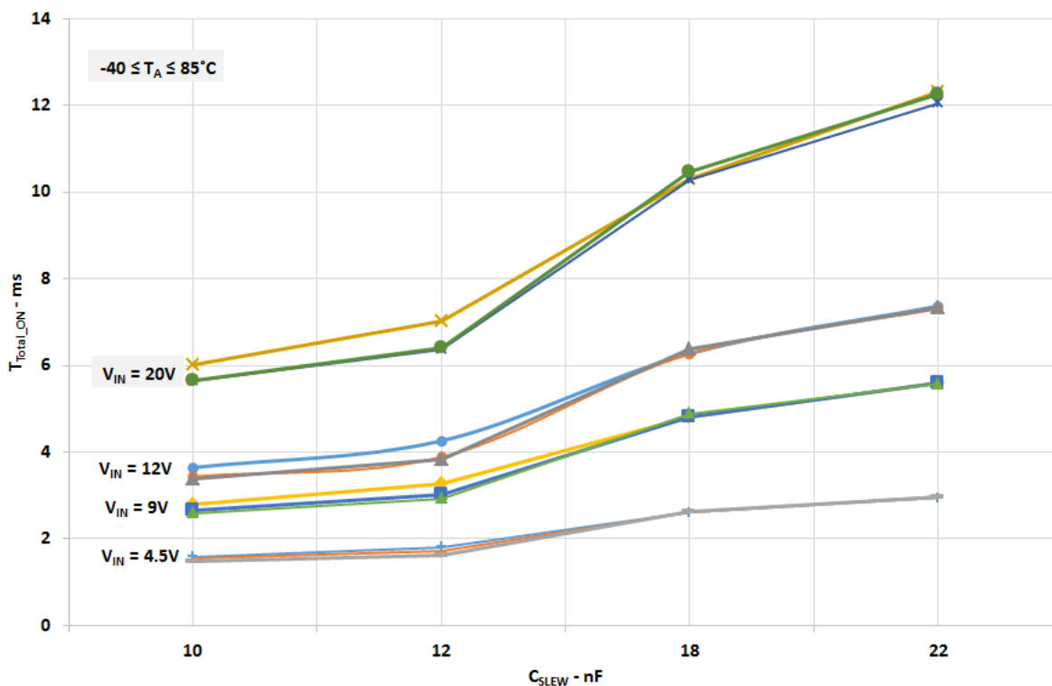
T Total_ON vs. C SLEW , V IN , and Temperature
