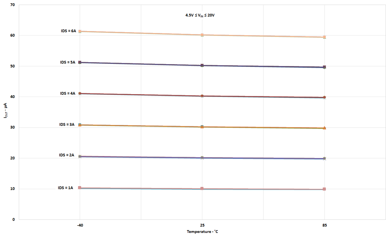
I_{OUT} vs. Temperature, MOSFET I_{DS} , and V_{IN}
