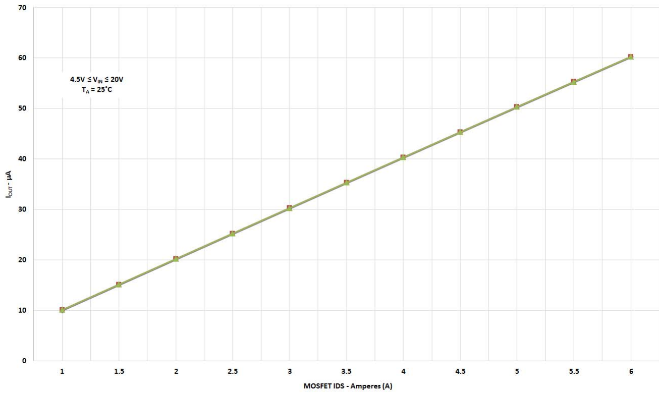
I_{OUT} vs. MOSFET I_{DS} and V_{IN}
