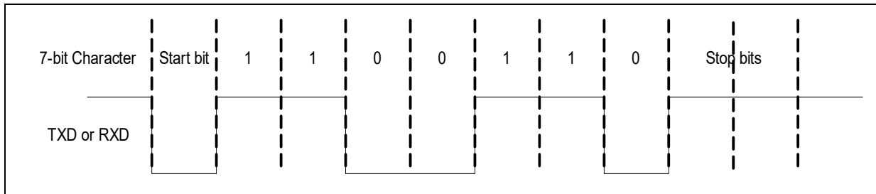
Figure 18-5. 7-bit Character Encoding
