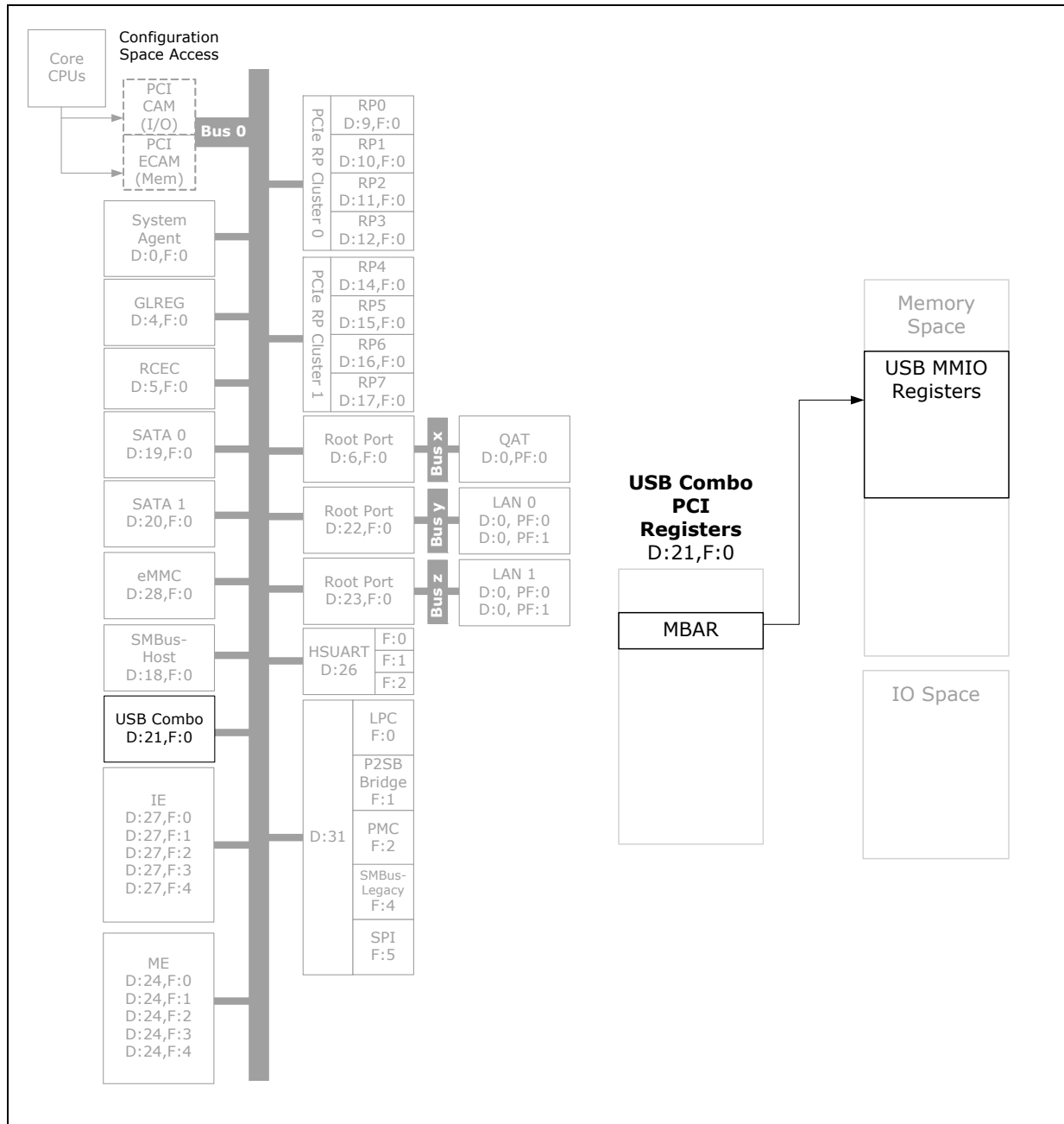
Figure 14-6. Register Map
