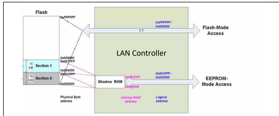
Figure 13-4. Shared SPI Flash Shadow RAM
