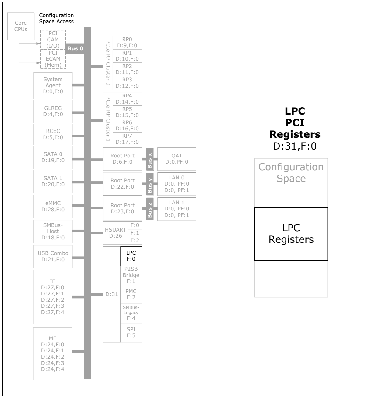
Figure 20-3. Register Map
