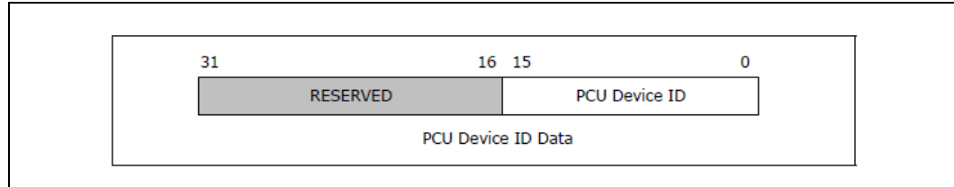
Figure 30-19. PCU Device ID Data
