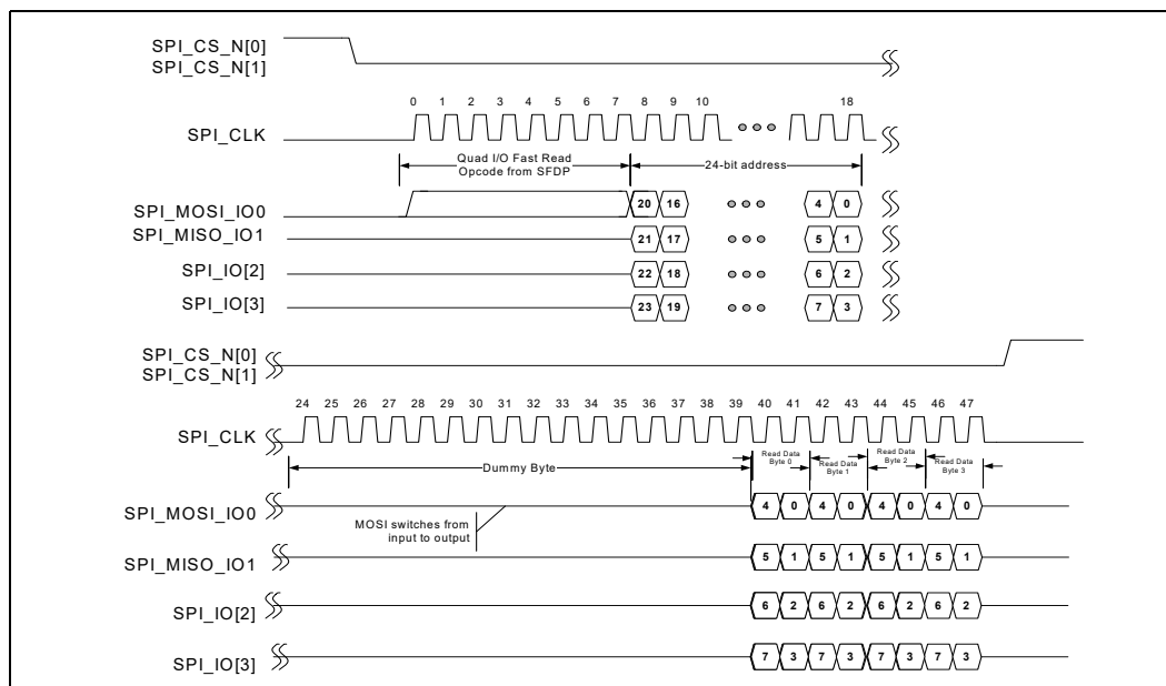
Figure 19-9. Quad-I/O-Fast-Read Timing
