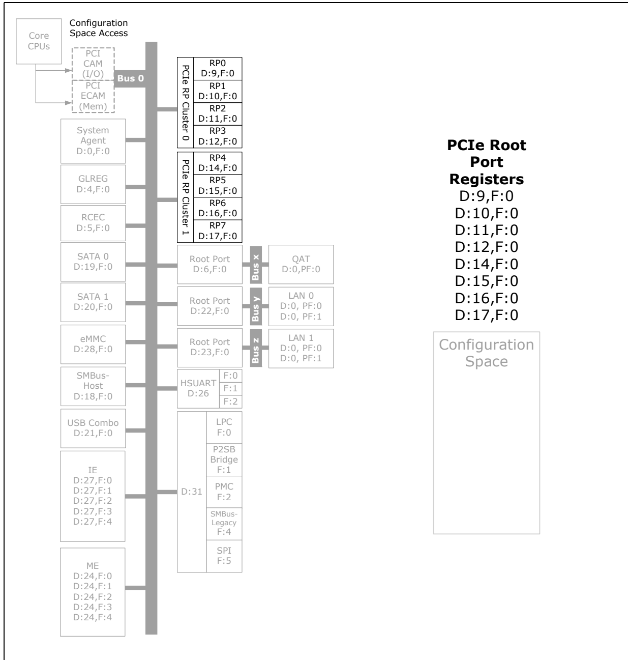
Figure 11-3. Register Map
