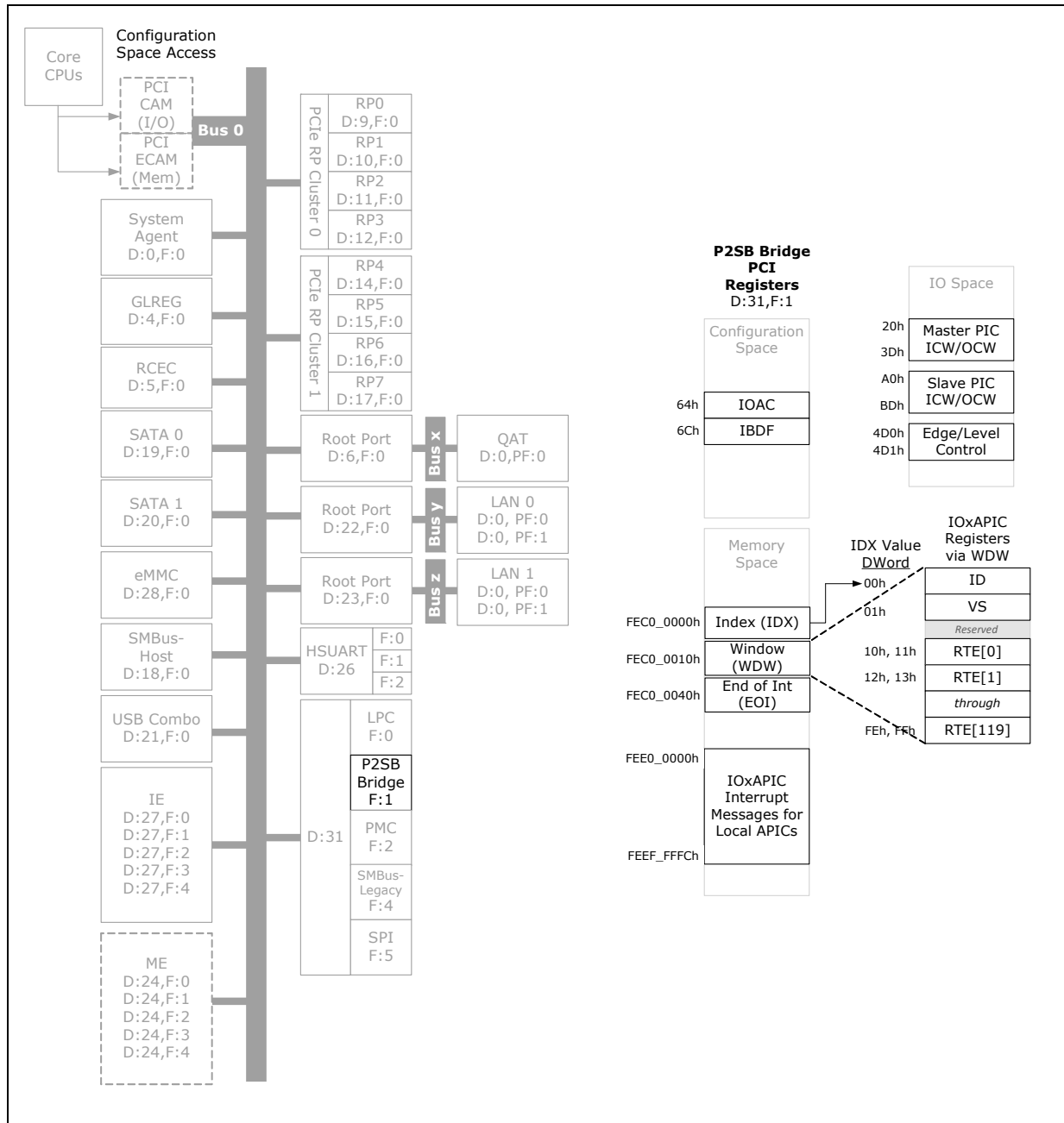
Figure 22-2. Register Map
