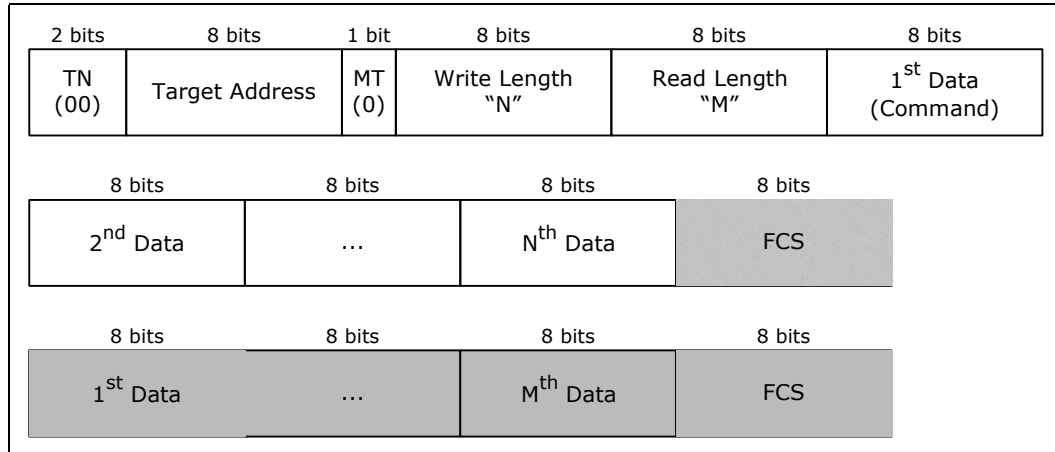
Figure 30-6. PEFI Write-Read Protocol
