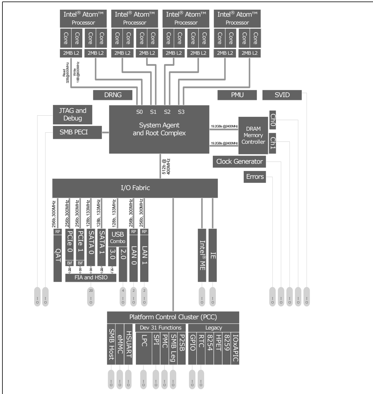
Figure 1-1. High-Level Block Diagram
