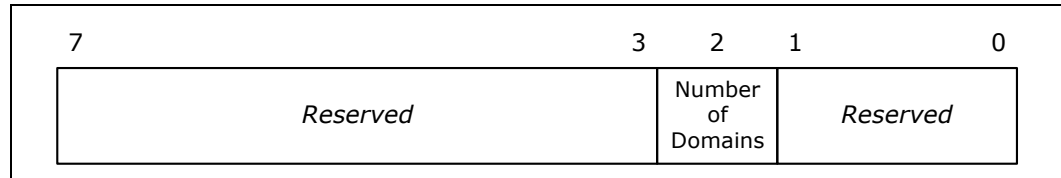
Figure 30-7. PECI Device Info Field Definition
