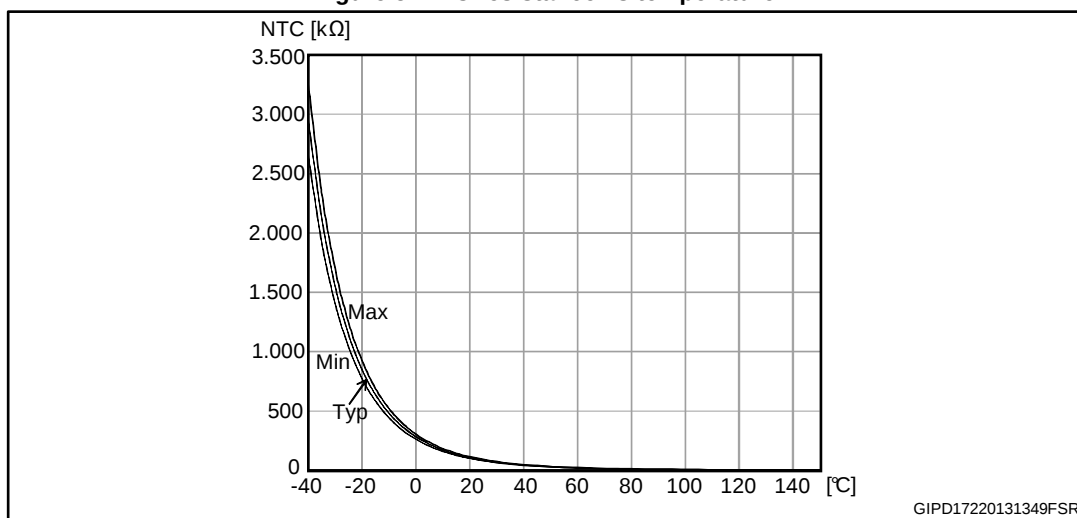
Figure 6: NTC resistance vs temperature (zoom)
