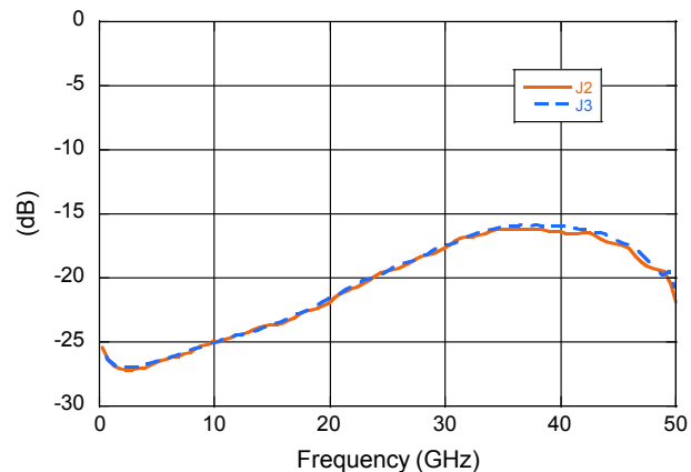
Output Return Loss @ -10 mA
