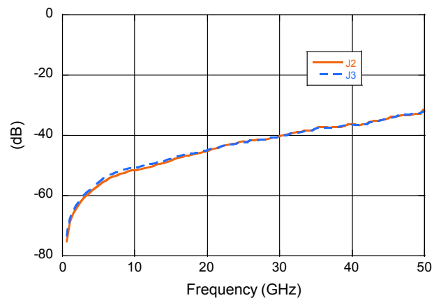
Isolation @ +10 mA
