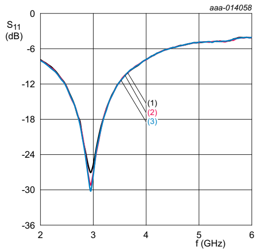
T_{amb} = 25 °C; gain mode (1) V_{CC} = V_{I(CTRL)} = 3.0 V (2) V_{CC} = V_{I(CTRL)} = 3.3 V (3) V_{CC} = V_{I(CTRL)} = 3.6 V
