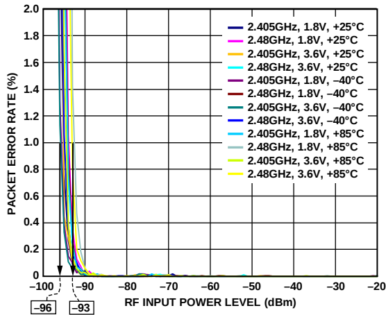
Figure 11. IEEE 802.15.4-2006 Packet Mode Sensitivity vs. Temperature and V_{DD\_BAT} , f_{CHANNEL} = 2.405\text{ GHz} , 2.45 GHz, 2.48 GHz, RFIO2x
