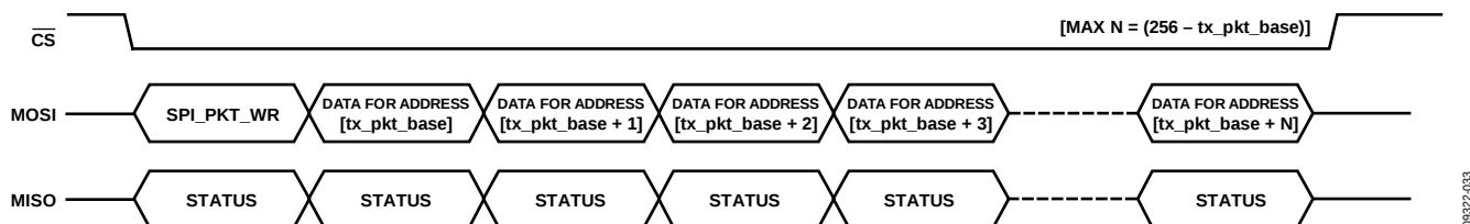
Figure 56. Packet RAM Write (tx_pkt_base is the address base pointer value for TX, which is programmed in Register txbp, Bit tx_pkt_base.)
