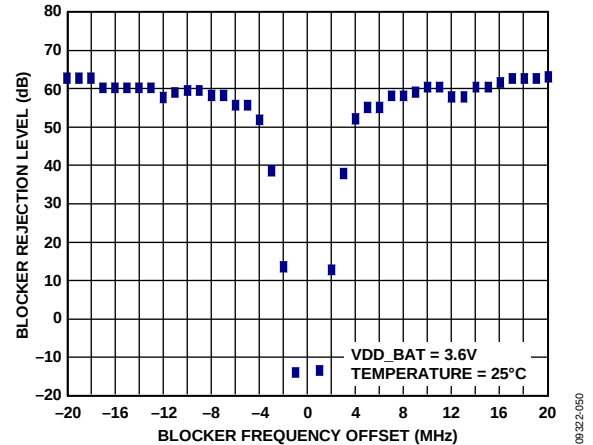
Figure 16. IEEE 802.15.4 Packet Mode Narrow-Band Blocker Rejection, CW Blocker, P_{WANTED} = -95\text{ dBm} + 3\text{ dB} , f_{CHANNEL} = 2.45\text{ GHz} , RFIO2x
