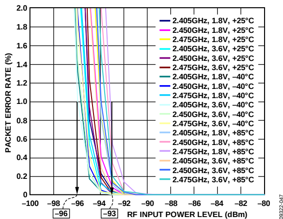
Figure 13. IEEE 802.15.4 Packet Mode Sensitivity vs. Temperature and V_{DD\_BAT} , f_{CHANNEL} = 2.405\text{ GHz} , 2.45 GHz, 2.475 GHz, RFIO1x
