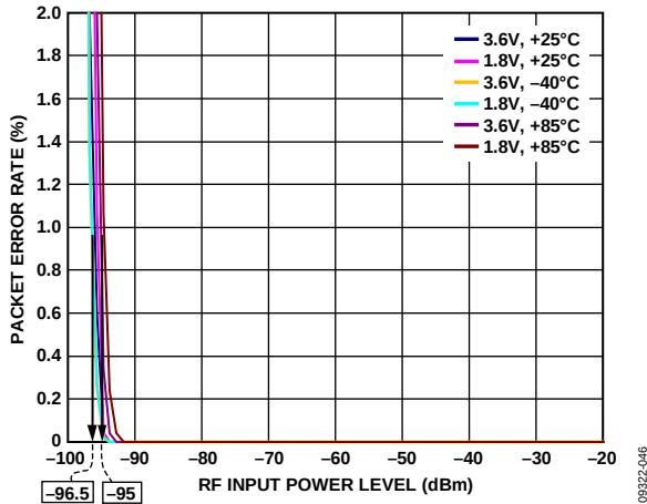
Figure 12. IEEE 802.15.4-2006 Packet Mode PER vs. RF Input Power Level vs. Temperature and V_{DD\_BAT} , f_{CHANNEL} = 2.45\text{ GHz} , RFIO2x
