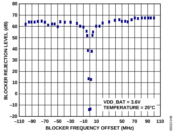
Figure 15. IEEE 802.15.4-2006 Packet Mode Wide-Band Blocker Rejection, CW Blocker, P_{WANTED} = -95\text{ dBm} + 3\text{ dB} , f_{CHANNEL} = 2.45\text{ GHz} , RFIO2x
