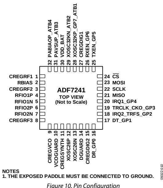
Figure 10. Pin Configuration
