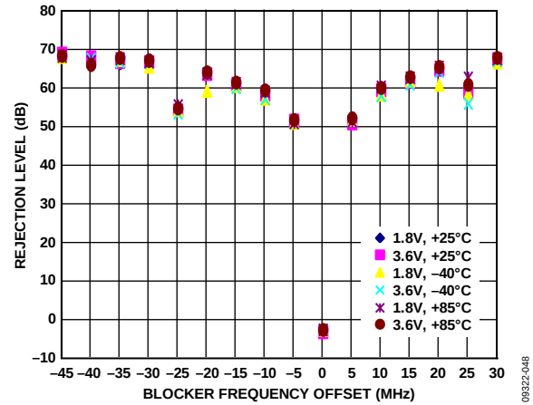
Figure 14. IEEE 802.15.4-2006 Packet Mode Blocker Rejection vs. Temperature and V_{DD\_BAT} , Modulated Blocker, P_{WANTED} = -85\text{ dBm} + 3\text{ dB} , f_{CHANNEL} = 2.45\text{ GHz} , RFIO2x
