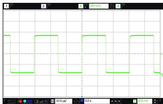
Figure 14. LVCMOS Output Waveform ( V_{\text{Swing}} = 1.8\text{V} , SiT1552AI-JE-DCC-32.768, 10 pF Load)
