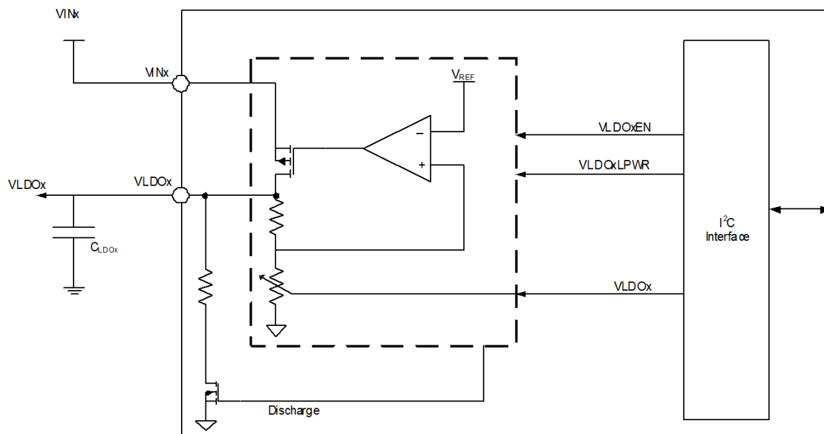
Figure 11. General LDO block diagram
