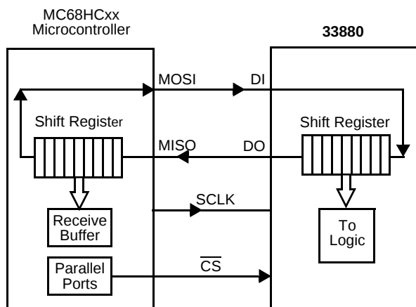
Figure 21. SPI Interface with Microcontroller
