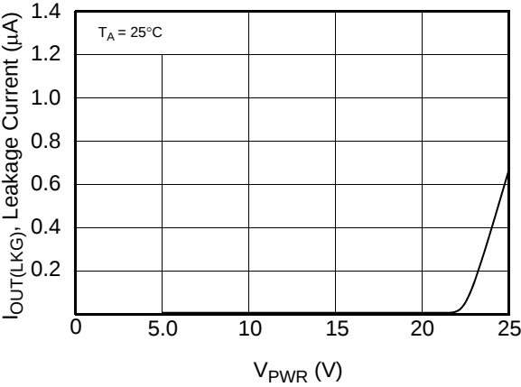
Figure 20. Sleep State Output Leakage vs. V_{PWR}
