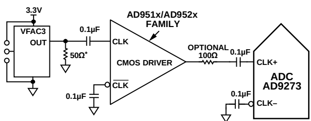
Figure 58. Single-Ended 1.8 V CMOS Sample Clock
