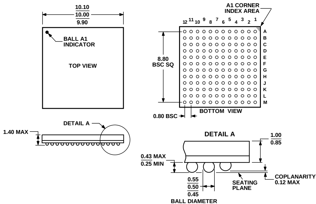
Figure 72. 144-Ball Chip Scale Package, Ball Grid Array [CSP_BGA] (BC-144-1) Dimensions shown in millimeters
