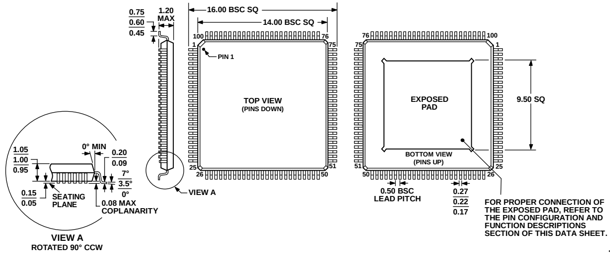
Figure 71. 100-Lead Thin Quad Flat Package, Exposed Pad [TQFP_EP] (SV-100-3) Dimensions shown in millimeters
