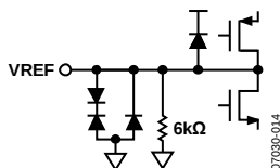
Figure 33. Equivalent VREF Circuit
