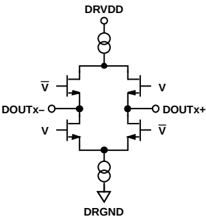
Figure 29. Equivalent Digital Output Circuit
