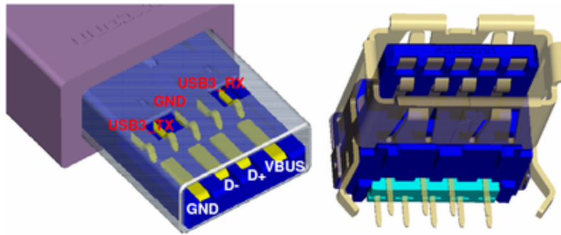
Figure 6 : USB 3.0 Standard-A Connector USB 3.0 Standard-A plug and receptacle. Image courtesy of USB Implementers Forum
