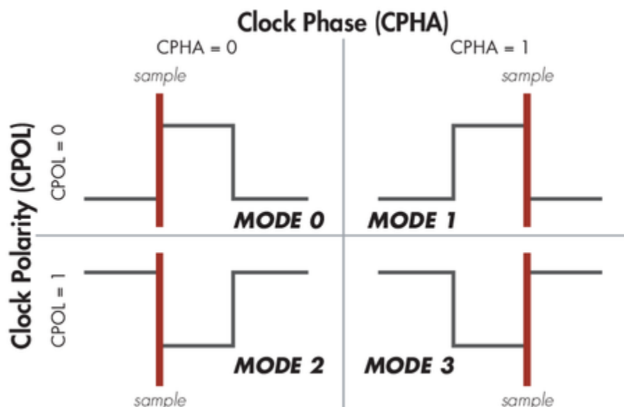
Figure 26 : SPI Modes
