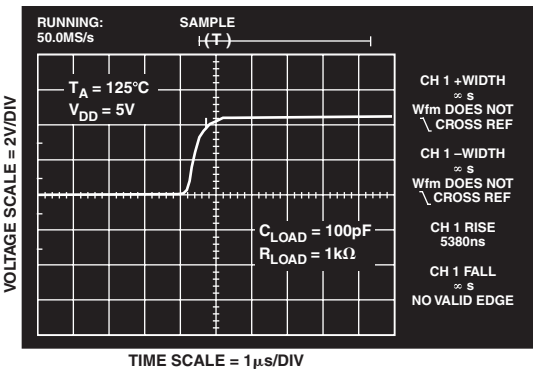
TPC 6. TMP03 Output Rise Time at 125^\circ C
