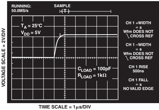
TPC 5. TMP03 Output Rise Time at 25^\circ C
