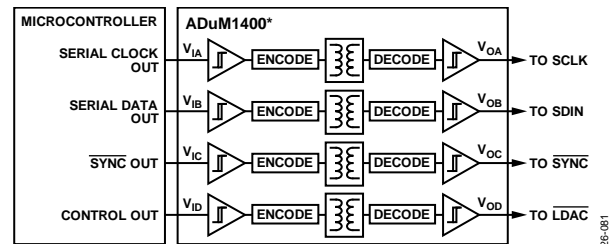
Figure 88. Isolated Interface
