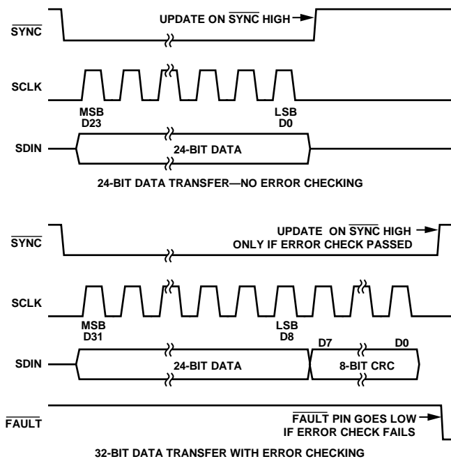
Figure 78. PEC Timing
