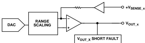
Figure 72. Voltage Output
