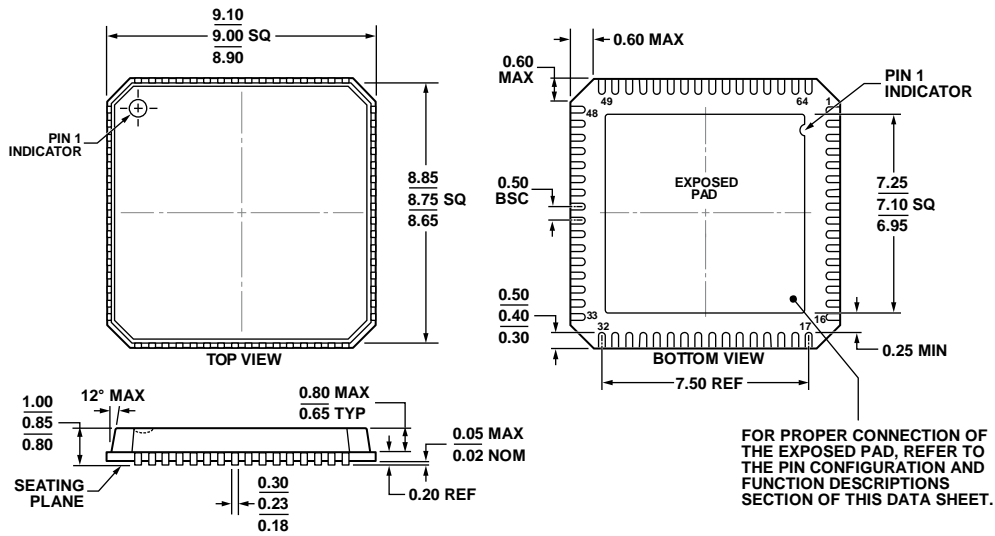
COMPLIANT TO JEDEC STANDARDS MO-220-VMM4 Figure 90. 64-Lead Lead Frame Chip Scale Package [LFCSP_VQ] 9 mm × 9 mm Body, Very Thin Quad (CP-64-3) Dimensions shown in millimeters
