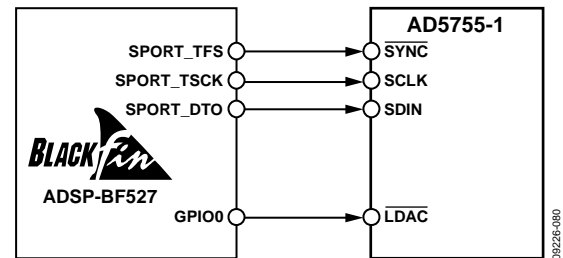
Figure 87. AD5755-1-to-ADSP-BF527 SPORT Interface
