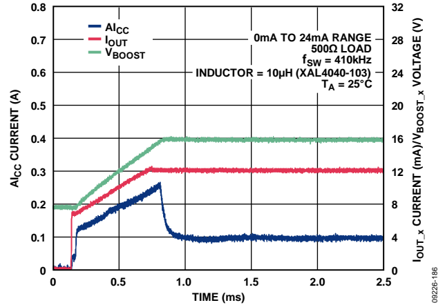
Figure 84. A_{I_{CC}} Current vs. Time for 24 mA Step Through 500 \Omega Load with External 51 k \Omega Compensation Resistor
