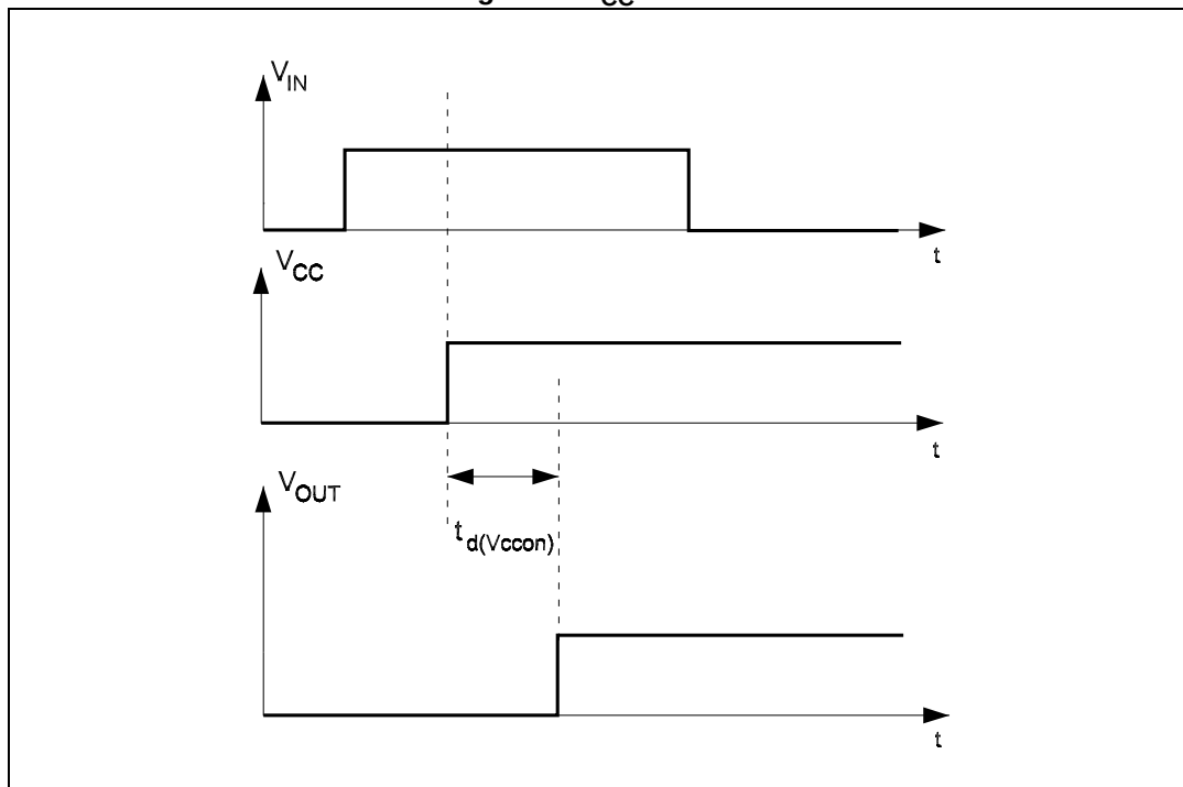
Figure 5. V_{CC} turn-ON
