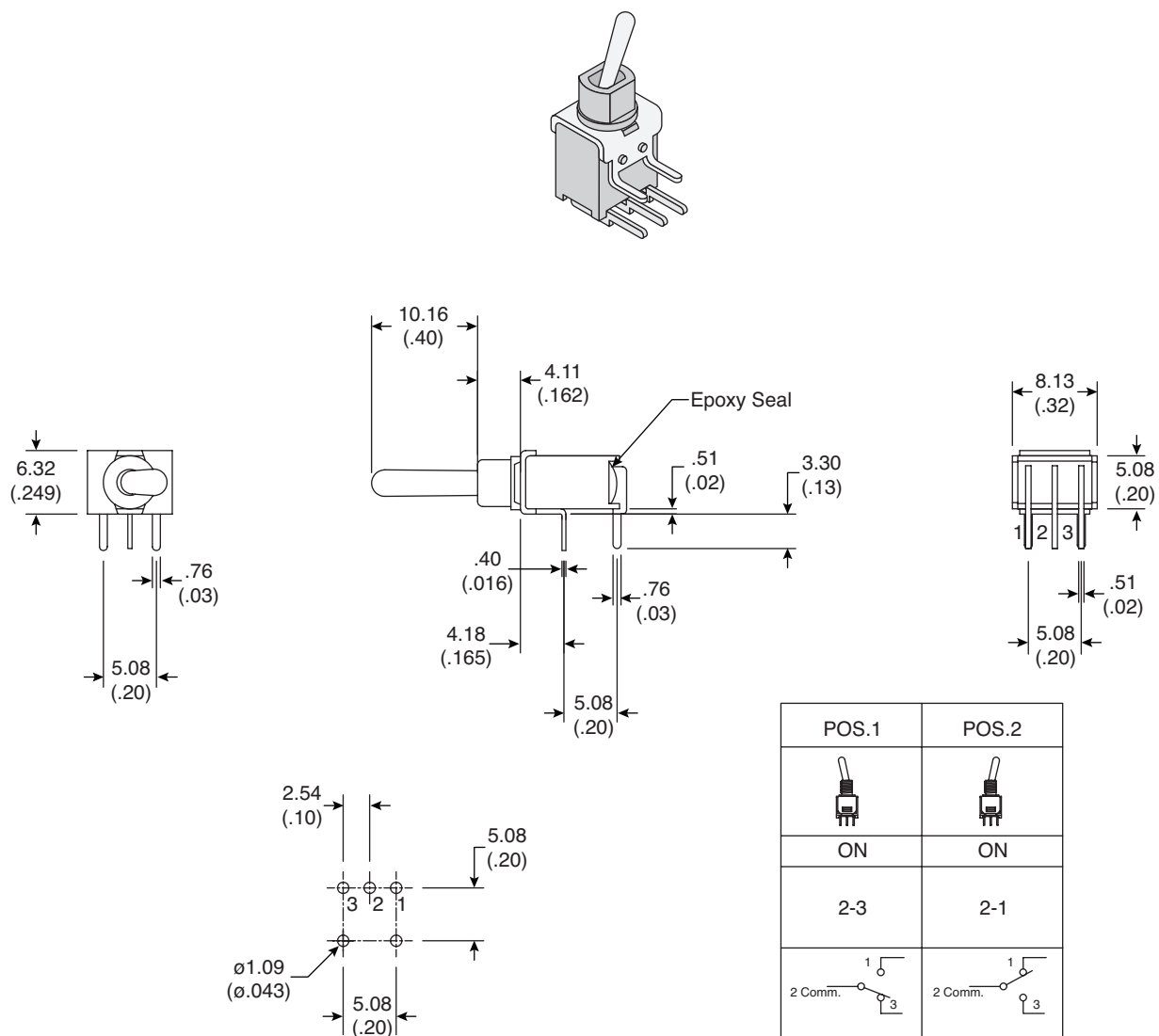
P.C. Mounting
