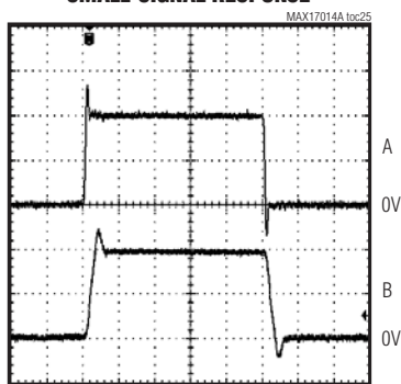
A: INPUT SIGNAL, 200mV/div B: OUTPUT SIGNAL, 200mV/div
