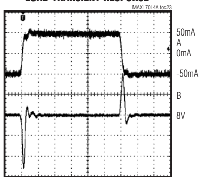
A: OUTPUT CURRENT, 50mA/div B: OUTPUT VOLTAGE, 500mV/div
