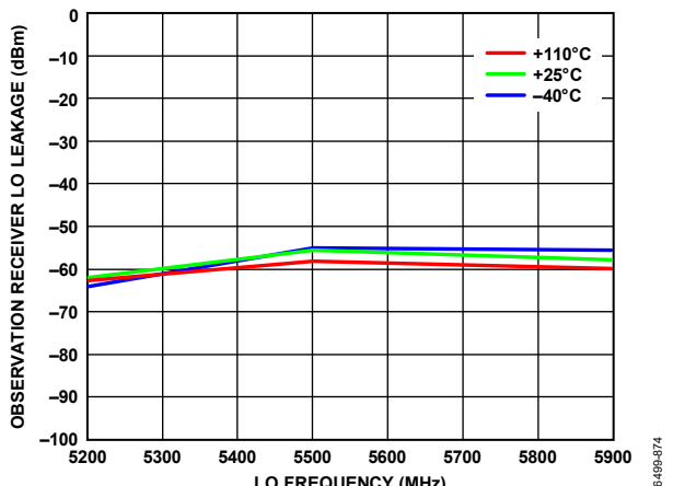
Figure 375. Observation Receiver LO Leakage vs. LO Frequency LO = 5200 MHz, 5500 MHz, and 5900 MHz
