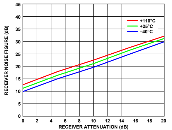
Figure 82. Receiver Noise Figure vs. Receiver Attenuation, LO = 75 MHz, RF Bandwidth = 50 MHz, Sample Rate = 61.44 MSPS, Integration Bandwidth = 1 MHz to 25 MHz
