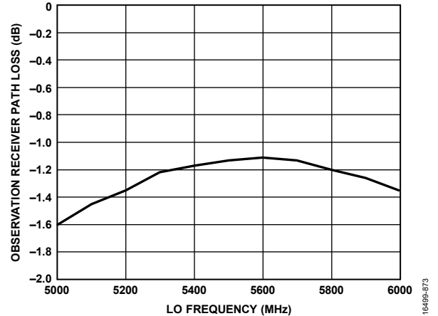
Figure 374. Observation Receiver Path Loss vs. LO Frequency, Can be Used for De-Embedding Performance Data
