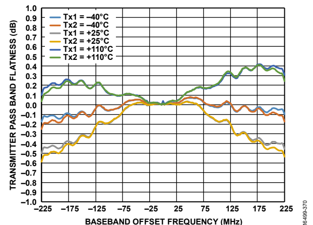
Figure 245. Transmitter Pass Band Flatness vs. Baseband Offset Frequency, Off Chip Match Response De-Embedded, LO = 4600 MHz
