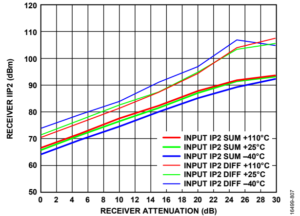
Figure 304. Receiver IIP2 vs. Receiver Attenuation, LO = 3600 MHz, Tones Placed at 3645 MHz and 3646 MHz, -21 dBm Plus Attenuation
