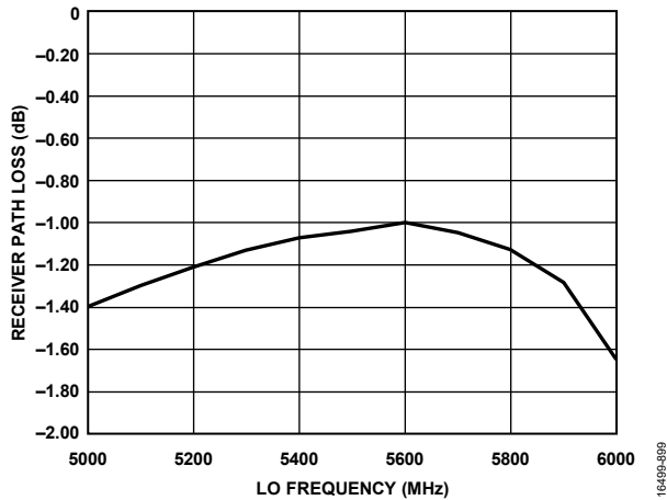
Figure 400. Receiver Path Loss vs. LO Frequency, Can Be Used for De-Embedding Performance Data
