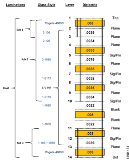
Figure 432. ADRV9009-W/PCBZ Trace Impedance and Stackup
