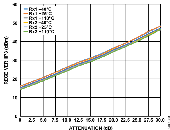
Figure 215. Receiver IIP3 vs. Attenuation, LO = 1800 MHz, Tone 1 = 1802 MHz, Tone 2 = 1892 MHz, -21 dBm Each at Attenuation = 0 dB
