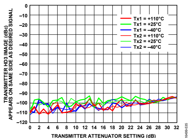
Figure 32. Transmitter HD3 Image Appears on Same Side as Desired Signal vs. Transmitter Attenuator Setting, LO = 300 MHz, CW = -15 dBFS
