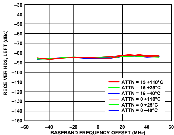
Figure 418. Receiver HD2, Left vs. Baseband Frequency Offset, Tone Level = -15 dBm at Attenuation = 0 dB, X-Axis = Baseband Frequency Offset of the Fundamental Tone, Not the Frequency of the HD2 Product (HD2 Product = 2 \times the Baseband Frequency), HD2 Canceller Disabled, LO = 5200 MHz
