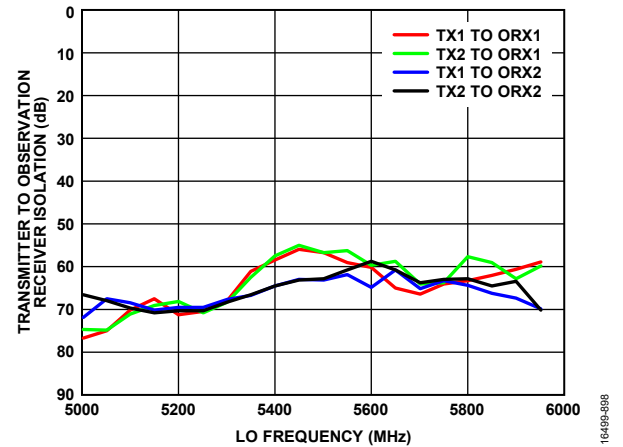
Figure 399. Transmitter to Observation Receiver Isolation vs. LO Frequency, Temperature = 25°C
