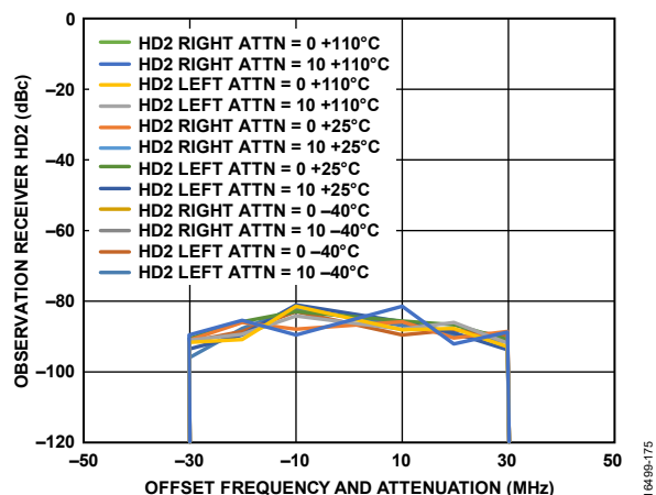
Figure 72. Observation Receiver HD2 vs. Offset Frequency and Attenuation, LO = 75 MHz, Tone Level = -21 dBm Plus Attenuation
