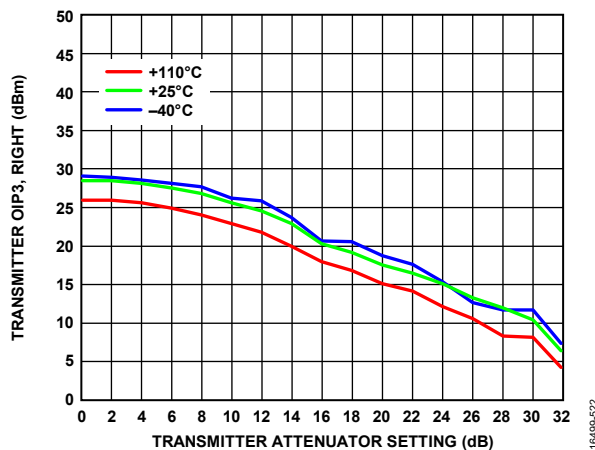
Figure 19. Transmitter OIP3 Right vs. Transmitter Attenuator Setting, LO = 75 MHz, Total Root Mean Square (RMS) Power = -12 dBFS, 20 MHz/25 MHz Tones
