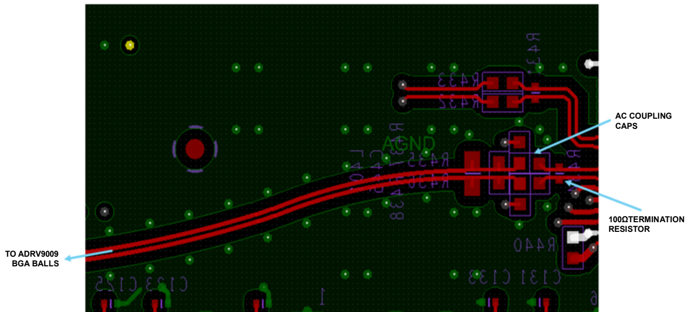
Figure 435. REF_CLK_IN± Routing Recommendation
