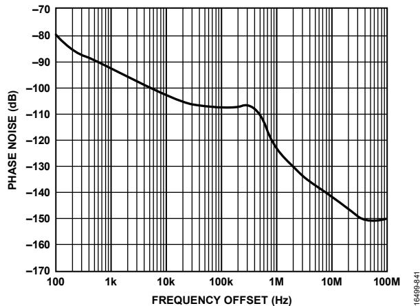
Figure 339. Phase Noise vs. Frequency Offset, LO = 3800 MHz, RMS Phase Error Integrated from 2 kHz to 18 MHz, PLL Loop Bandwidth = 300 kHz, Spectrum Analyzer Limits Far Out Noise
