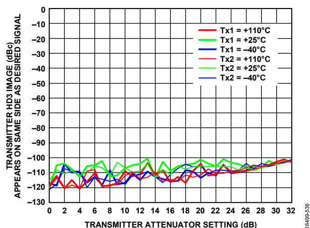
Figure 33. Transmitter HD3 Image Appears on Same Side as Desired Signal vs. Transmitter Attenuator Setting, LO = 525 MHz, CW = -15 dBFS
