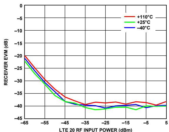
Figure 423. Receiver EVM vs. LTE20 RF Input Power, LO = 5500 MHz, Default AGC Settings
