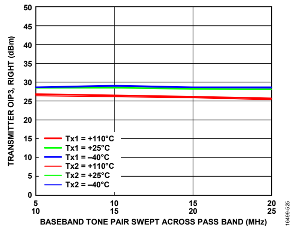
Figure 22. Transmitter OIP3 Right vs. Baseband Tone Pair Swept Across Pass Band, LO = 75 MHz, Total RMS Power = -12 dBFS, Transmitter Attenuation = 4 dB
