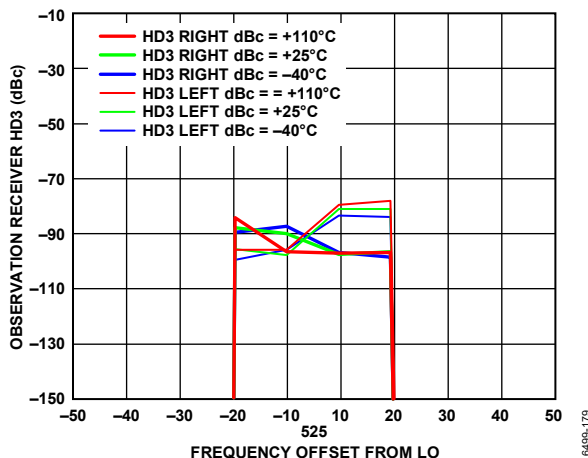
Figure 76. Observation Receiver HD3 vs. Frequency Offset from LO, Tone Level = -22 dBm at Attenuation = 0 dB, LO = 525 MHz
