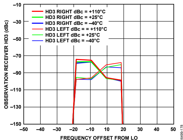
Figure 75. Observation Receiver HD3 vs. Frequency Offset from LO, Tone Level = -22 dBm at Attenuation = 0 dB, LO = 300 MHz
