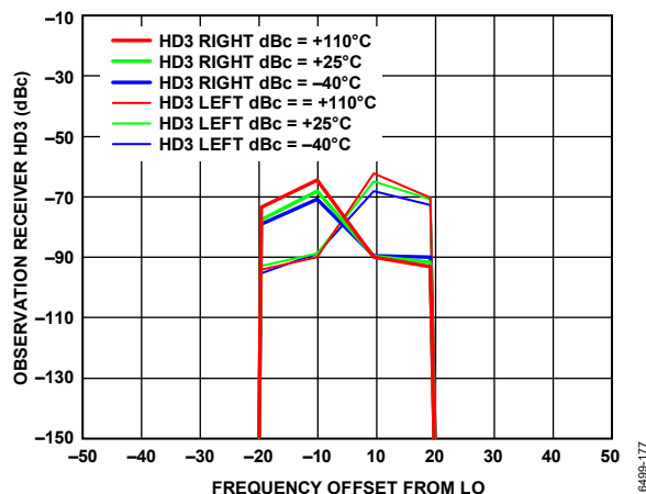
Figure 74. Observation Receiver HD3 vs. Frequency Offset from LO, Tone Level = -21 dBm at Attenuation = 0 dB, LO = 75 MHz
