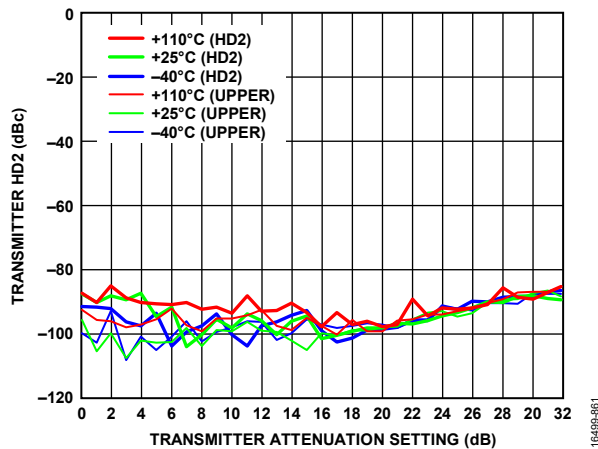
Figure 359. Transmitter HD2 vs. Transmitter Attenuator Setting, Baseband Frequency = 10 MHz, LO = 5100 MHz, CW = -15 dBFS
