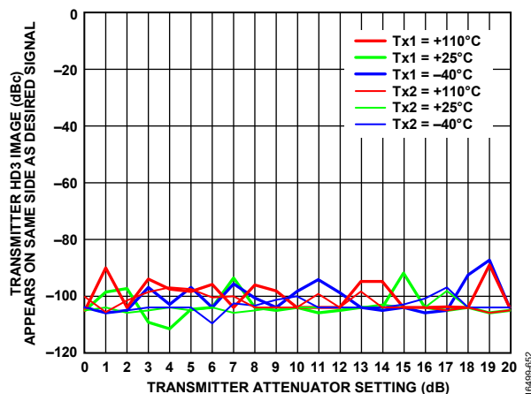
Figure 149. Transmitter HD3 Image Appears on Same Sideband as Desired Signal vs. Transmitter Attenuator Setting, LO = 1850 MHz Digital Backoff = 15 dB
