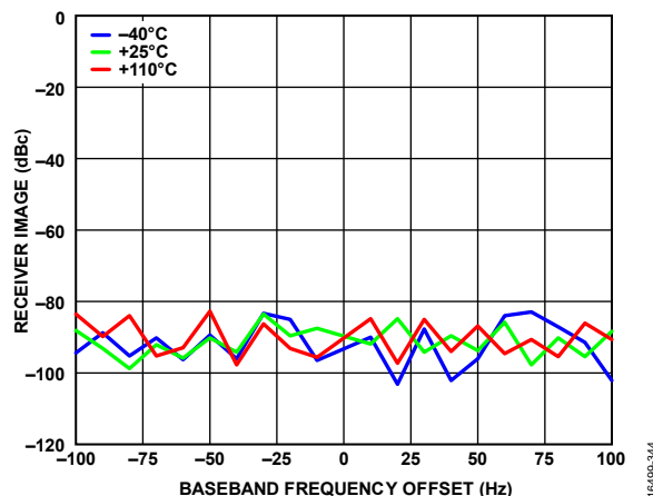
Figure 221. Receiver Image vs. Baseband Frequency Offset, Attenuation = 0 dB, RF Bandwidth = 200 MHz, Tracking Calibration Active, Sample Rate = 245.76 MSPS, LO = 2850 MHz
