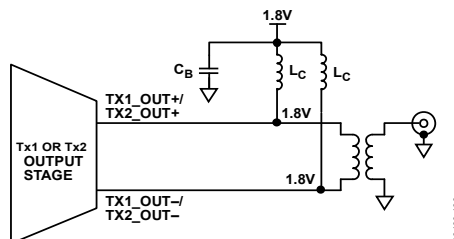
Figure 458. Using Bias Chokes and a Transformer
