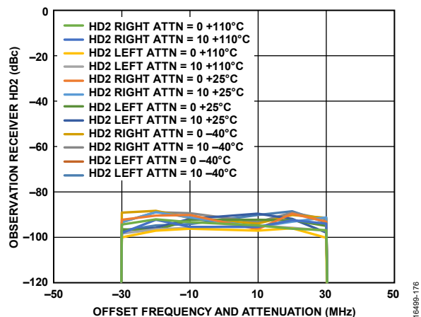
Figure 73. Observation Receiver HD2 vs. Offset Frequency and Attenuation, LO = 300 MHz, Tone Level = -22 dBm Plus Attenuation
