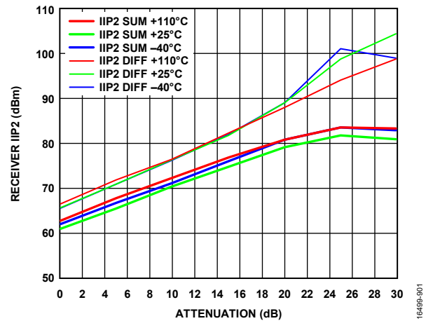
Figure 402. Receiver IIP2 vs. Attenuation, LO = 5800 MHz LO, Tones Placed at 5845 MHz and 5846 MHz, -21 dBm Plus Attenuation
