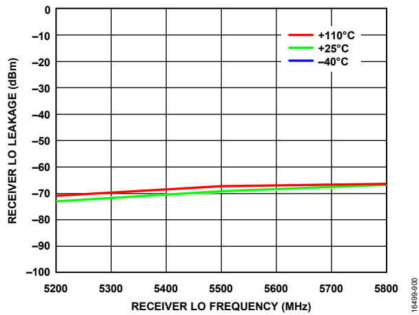
Figure 401. Receiver LO Leakage vs. Receiver LO Frequency, LO = 5200 MHz, 5500 MHz, and 5800 MHz, Receiver Attenuation = 0 dB, RF Bandwidth = 200 MHz, Sample Rate = 245.76 MSPS
