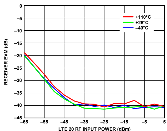
Figure 422. Receiver EVM vs. LTE20 RF Input Power, LO = 5200 MHz, Default AGC Settings
