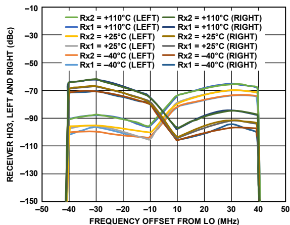
Figure 421. Receiver HD3, Left and Right vs. Frequency Offset from LO, Tone Level = -15 dBm at Attenuation = 0 dB, LO = 5900 MHz
