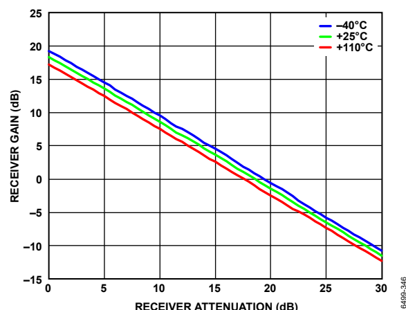
Figure 223. Receiver Gain vs. Receiver Attenuation, RF Bandwidth = 20 MHz, Sample Rate = 245.76 MSPS, LO = 1850 MHz
