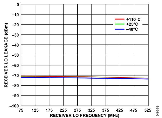
Figure 81. Receiver LO Leakage vs. Receiver LO Frequency = 75 MHz, 300 MHz, and 525 MHz, Receiver Attenuation = 0 dB, RF Bandwidth = 50 MHz, Sample Rate = 61.44 MSPS
