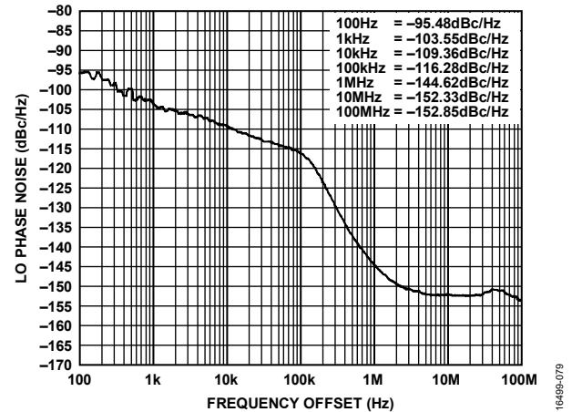
Figure 80. LO Phase Noise vs. Frequency Offset, LO = 525 MHz, PLL Loop Bandwidth = 50 kHz
