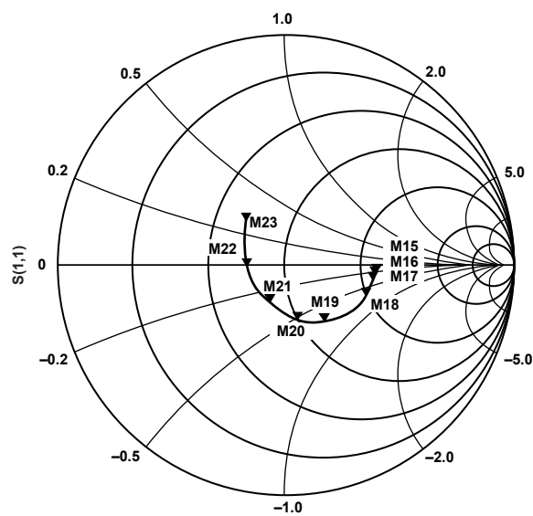
Figure 449. Receiver 1 and Receiver 2 SEDZ and PEDZ Data
