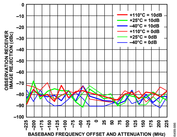
Figure 387. Observation Receiver Image Rejection vs. Baseband Frequency Offset and Attenuation, CW Signal Swept Across the Pass Band, LO = 5200 MHz
