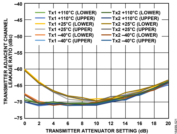
Figure 18. Transmitter Adjacent Channel Leakage Ratio vs. Transmitter Attenuator Setting, Signal Offset = 0 MHz, LO = 525 MHz, LTE = 20 MHz, PAR = 12 dB, DAC Boost Normal, Upper Side and Lower Side, Performance Limited by Spectrum Analyzer at Higher Attenuation Settings
