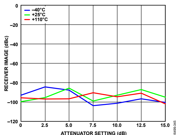
Figure 222. Receiver Image vs. Attenuator Setting, RF Bandwidth = 200 MHz, Tracking Calibration Active, Sample Rate = 245.76 MSPS, LO = 1850 MHz
