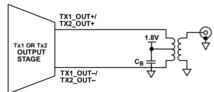
Figure 456. Using a Center Tapped Transformer
