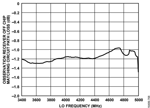
Figure 265. Observation Receiver Off Chip Matching Circuit Path Loss vs. LO Frequency, Simulation, Can be Used for De-Embedding Performance Data
