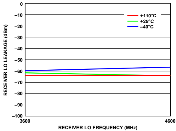
Figure 301. Receiver LO Leakage vs. Receiver LO Frequency, Receiver Attenuation = 0 dB, RF Bandwidth = 200 MHz, Sample Rate = 245.76 MSPS
