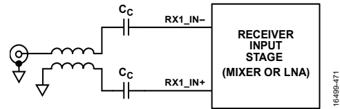
Figure 461. Differential Receiver Interface Using a Transmission Line Balun
