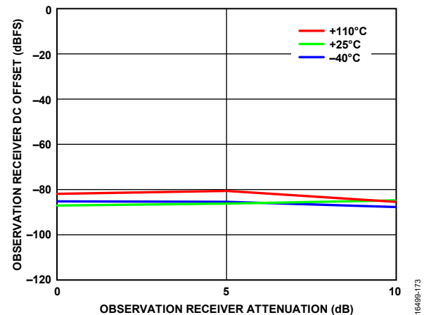
Figure 70. Observation Receiver DC Offset vs. Observation Receiver Attenuation, LO = 75 MHz, Baseband Frequency = 50 MHz
