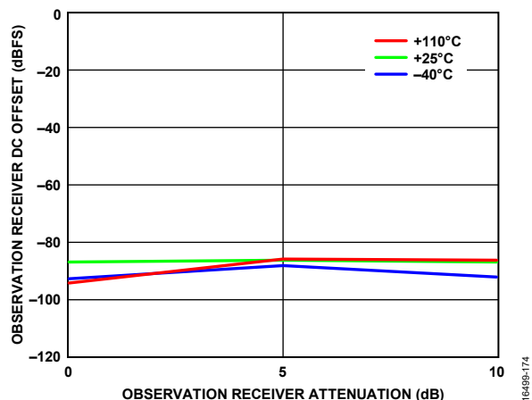
Figure 71. Observation Receiver DC Offset vs. Observation Receiver Attenuation, LO = 325 MHz, Baseband Frequency = 50 MHz
