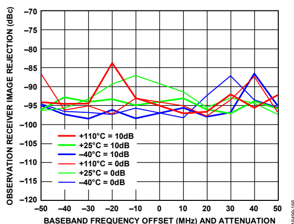
Figure 63. Observation Receiver Image Rejection vs. Baseband Frequency Offset and Attenuation, CW Signal Swept Across the Pass Band, LO = 300 MHz
