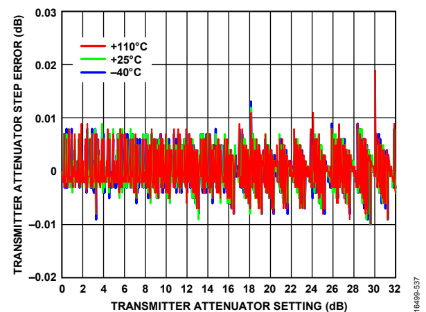
Figure 34. Transmitter Attenuator Step Error vs. Transmitter Attenuator Setting, LO = 75 MHz, Baseband Frequency = 10 MHz, Backoff = 15 dBFS
