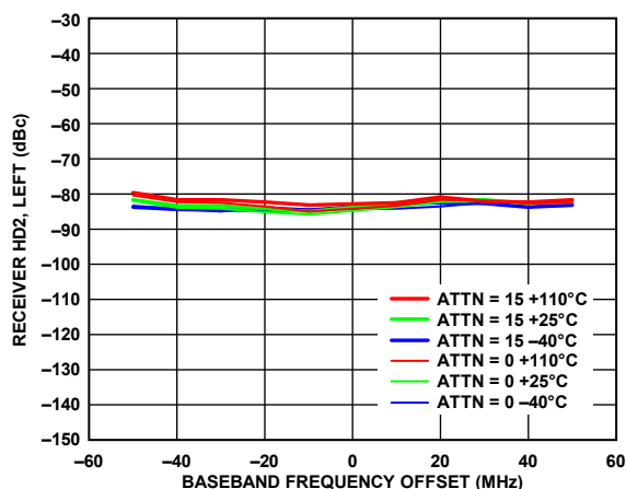
Figure 419. Receiver HD2, Left vs. Baseband Frequency Offset, Tone Level = -15 dBm at Attenuation = 0 dB, X-Axis = Baseband Frequency Offset of the Fundamental Tone, Not the Frequency of the HD2 Product (HD2 Product = 2 \times the Baseband Frequency), HD2 Canceller Disabled, LO = 5900 MHz
