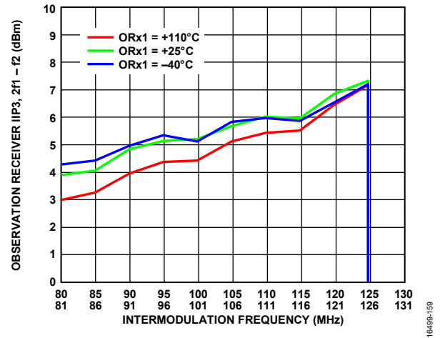
Figure 56. Observation Receiver IIP3, 2f_1 (Where 2f_1 is 2 \times f_1 ) - f_2 vs. Intermodulation Frequency, LO = 75 MHz, Attenuation = 0 dB, Tones Separated by 1 MHz Swept Across Pass Band at -25 dBm Each
