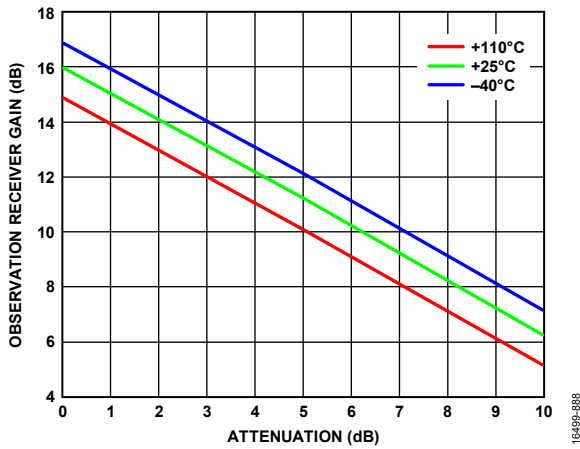
Figure 389. Observation Receiver Gain vs. Attenuation, LO = 5200 MHz
