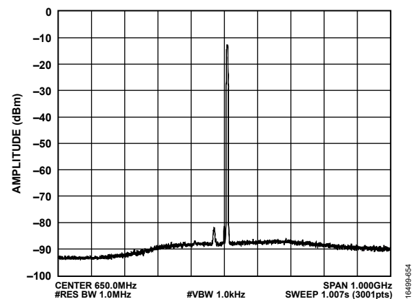
Figure 151. Amplitude vs. Frequency, Transmitter Output Spurious, Transmitter 1 = 650 MHz, LTE = 5 MHz, Offset = 10 MHz, RMS = -12 dBFS, Temperature = 25°C
