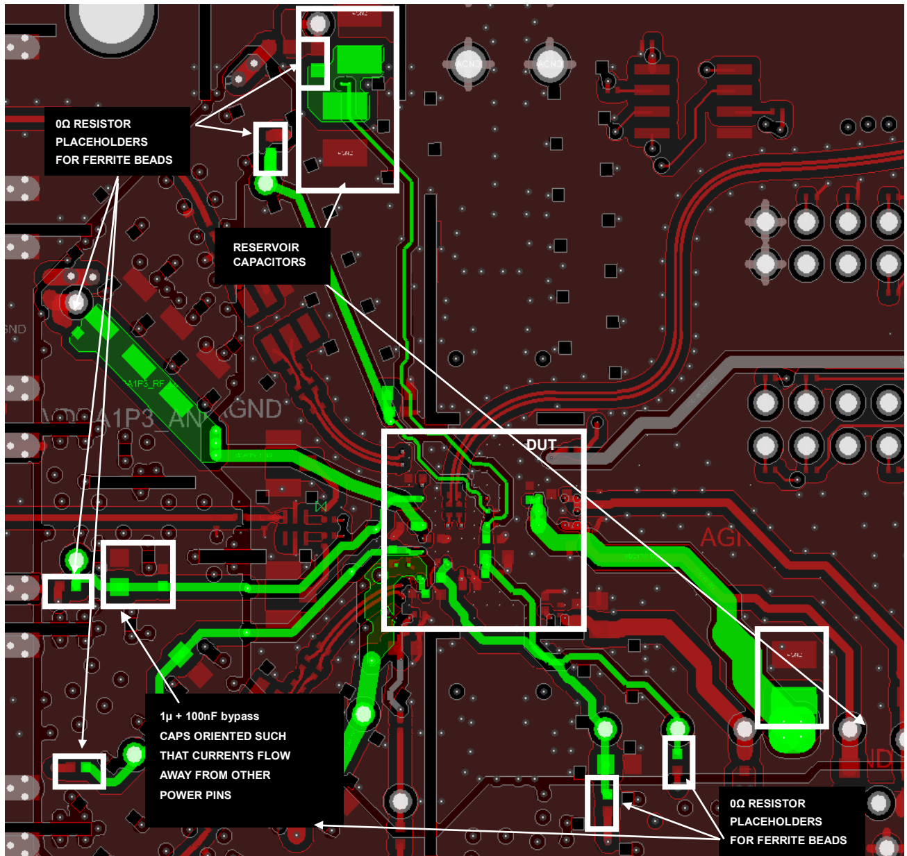
Figure 438. Placement Example of 0 \Omega Resistor Placeholders for FBs, Reservoir Capacitors, and Bypass Capacitors on the ADRV9009-W/PCBZ (Layer 12 to Power Layer and Bottom Layer)
