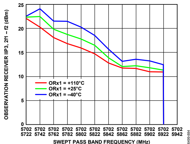
Figure 385. Observation Receiver IIP3, 2f_1 - f_2 vs. Swept Pass Band Frequency, LO = 5700 MHz, Tone 1 = 5702 MHz, Tone 2 = 5722 MHz at -22 dBm Each Plus Attenuation
