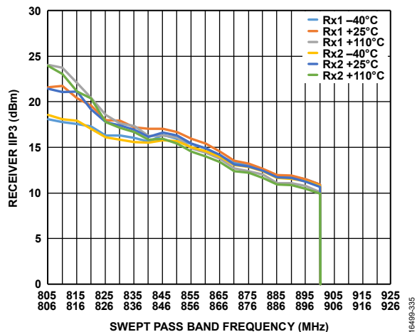
Figure 212. Receiver IIP3 vs. Swept Pass Band Frequency, Receiver Attenuation = 0 dB, LO = 800 MHz, Tone 2 = Tone 1 + 1 MHz, -21 dBm Each, Swept Across Pass Band
