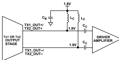
Figure 459. Using a Differential to Single-Ended Driver Amplifier
