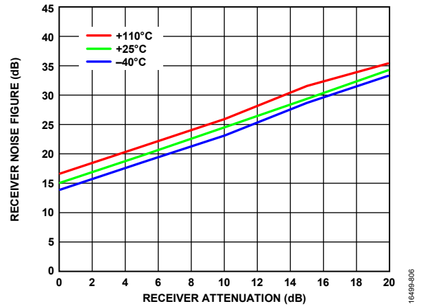
Figure 303. Receiver Noise Figure vs. Receiver Attenuation, LO = 4600 MHz, Bandwidth = 200 MHz, Sample Rate = 245.76 MSPS, Integration Bandwidth = 500 kHz to 100 MHz
