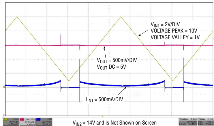
Figure 3. Transitioning from V_{IN1} to V_{IN2} and Back in PRIORITY Mode Operation with V_{IN2} at 14V
