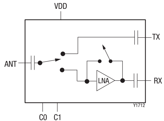
Figure 1. SKYA21041 Block Diagram
