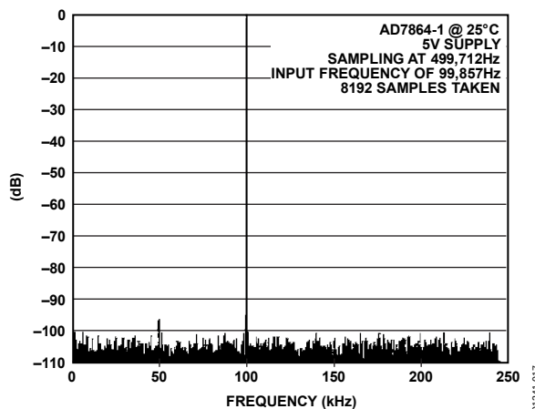
Figure 17. FFT Plot
