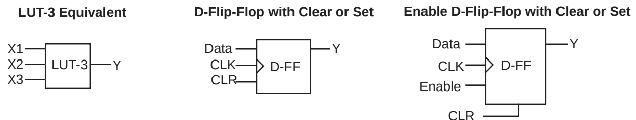
Figure 1-4 • VersaTile Configurations
