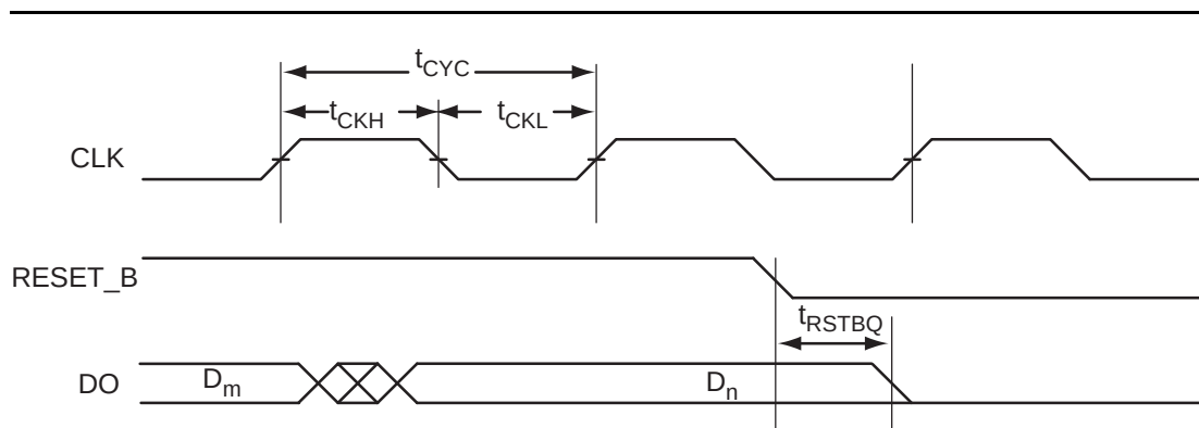
Figure 2-49 • RAM Reset
