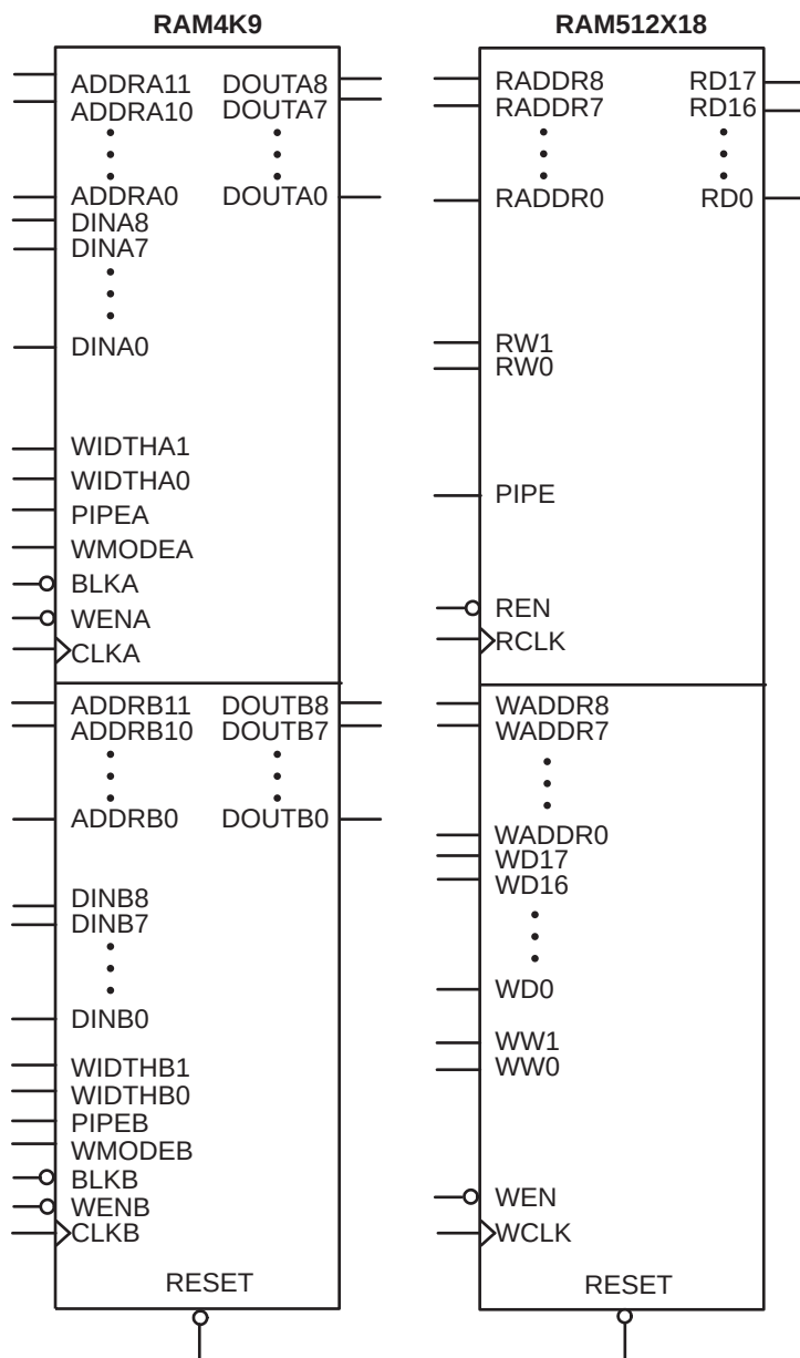
Figure 2-44 • RAM Models
