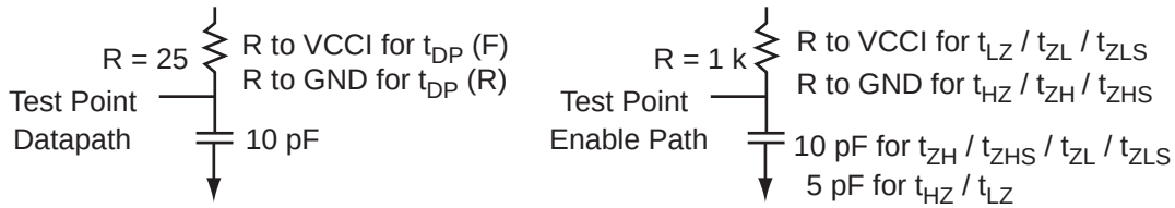
Figure 2-15 • AC Loading
