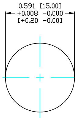
PANEL CUTOUT
