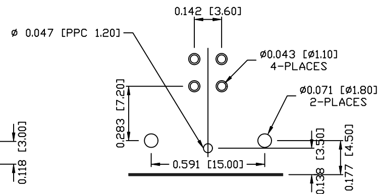
PLC LAYOUT
