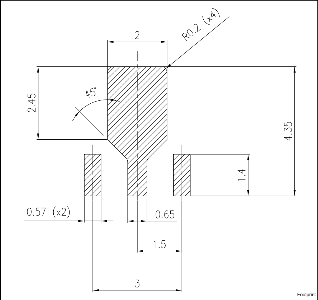
Figure 4. SOT-89 recommended footprint
