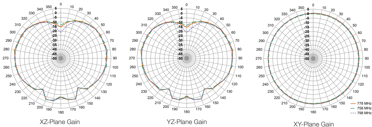
Figure9. Radiation Patterns for CW LTE Band 14 Antenna
