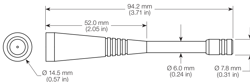
Figure 7. CW LTE Band 14 Antenna Dimensions
