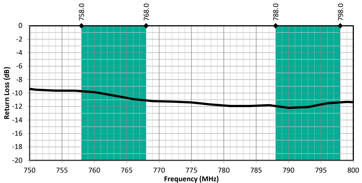
Figure3. CW LTE Band 14 Antenna Return Loss with Band 14 Uplink/Downlink Highlights
