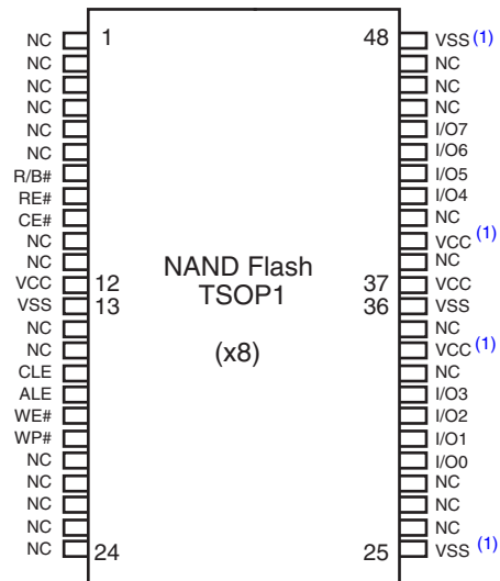
Figure 1.1 48-Pin TSOP1 Contact x8 Device (1 CE 8 Gb)
