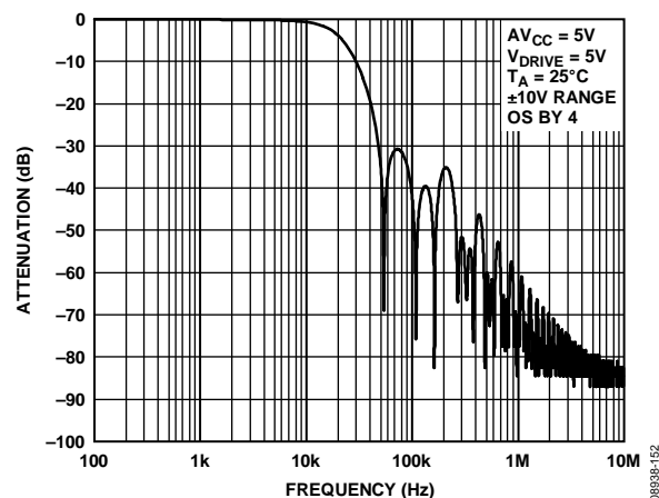
Figure 54. Digital Filter Response for OS \times 4
