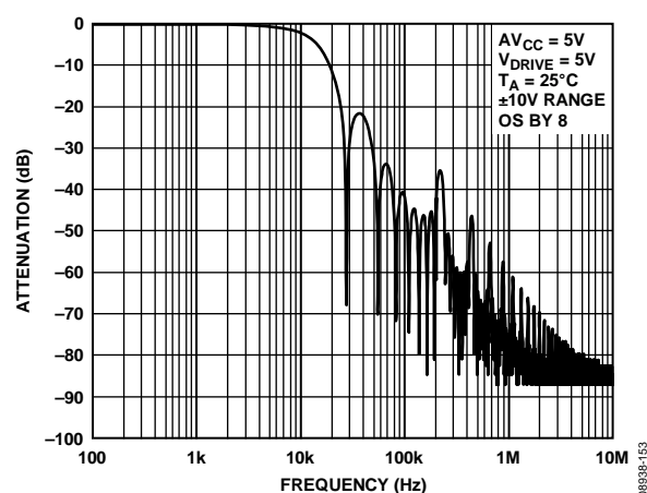
Figure 55. Digital Filter Response for OS \times 8
