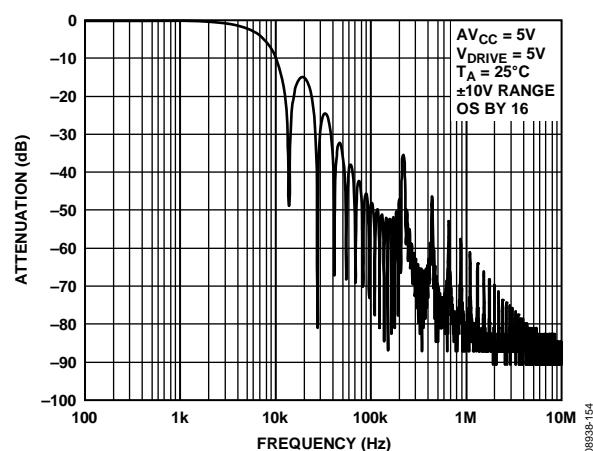
Figure 56. Digital Filter Response for OS \times 16
