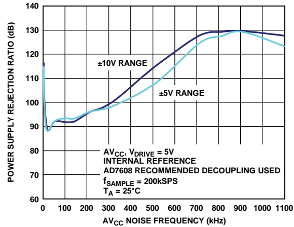
Figure 30. PSRR
