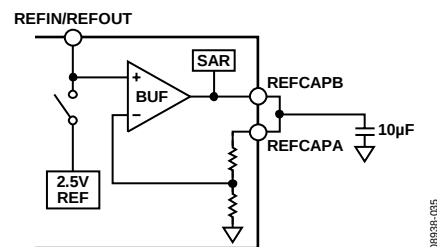
Figure 37. Reference Circuitry
